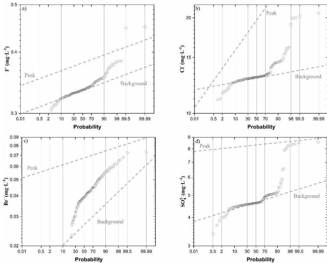
Online Resource 3.- Cumulative frequency plots of (A) F - , (B) Cl - , (C) Br - and (D) SO 4 2- of groundwater from Peña Horeb (PH) collected during the period 2017-2022. Dashed lines indicate the background and peak log-normal populations.
