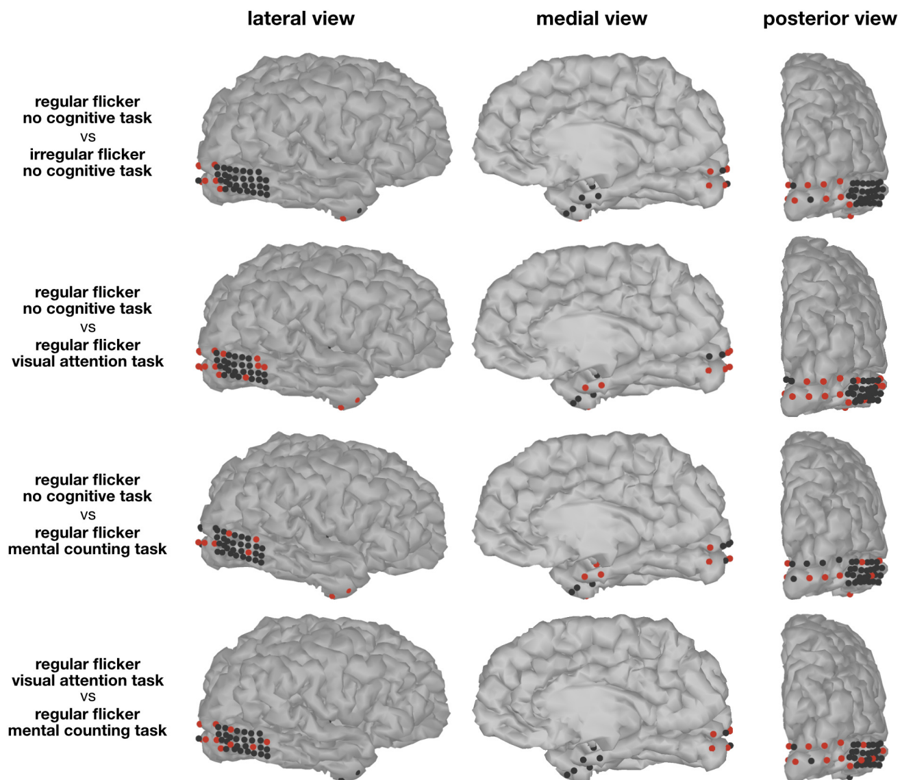
Figure S2. The results of multiple comparison on individual electrode of ECoG grids. The electrodes colored in red show significance for the comparison specified on the left side of the figure.
