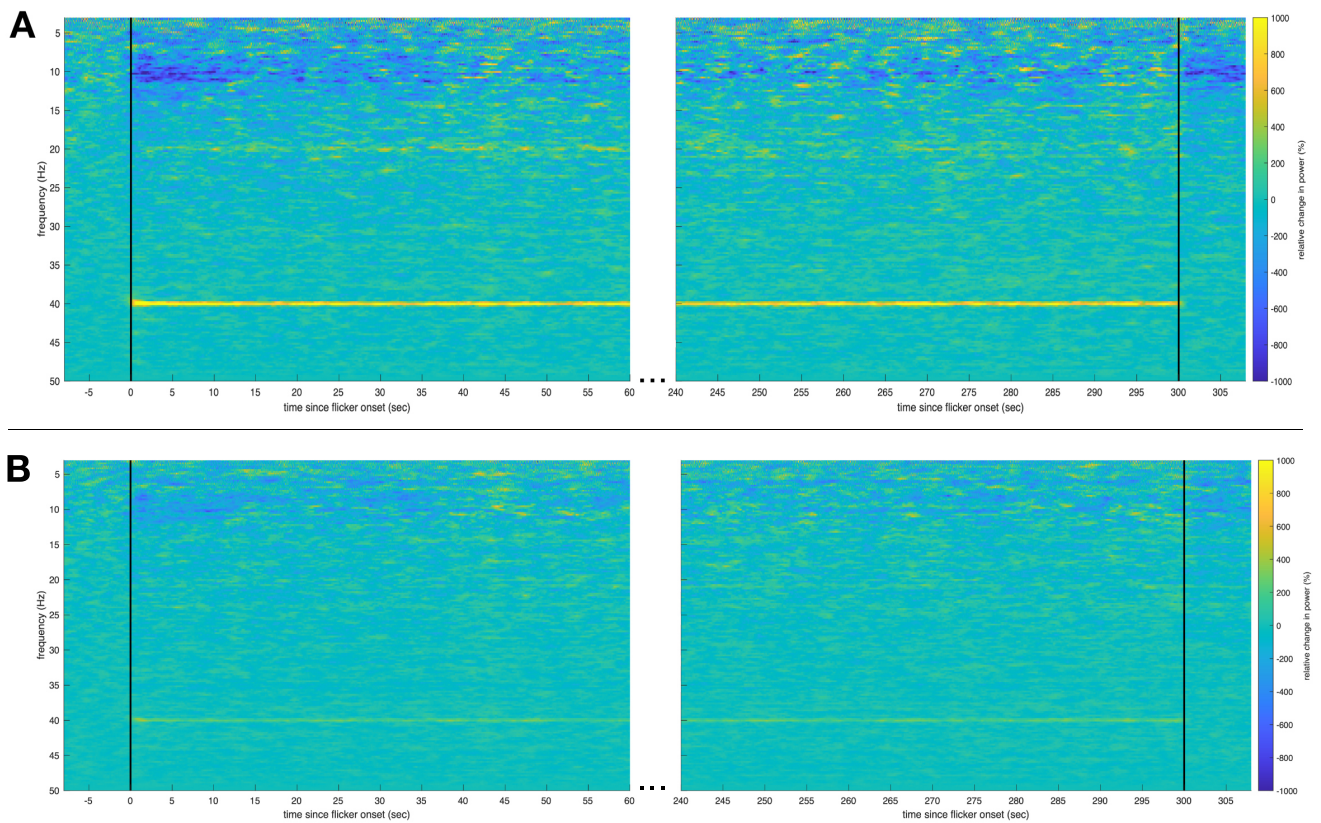
Figure S1. Time frequency analysis of the no-task condition with regular flickering at channel (A) Oz and (B) CPz
