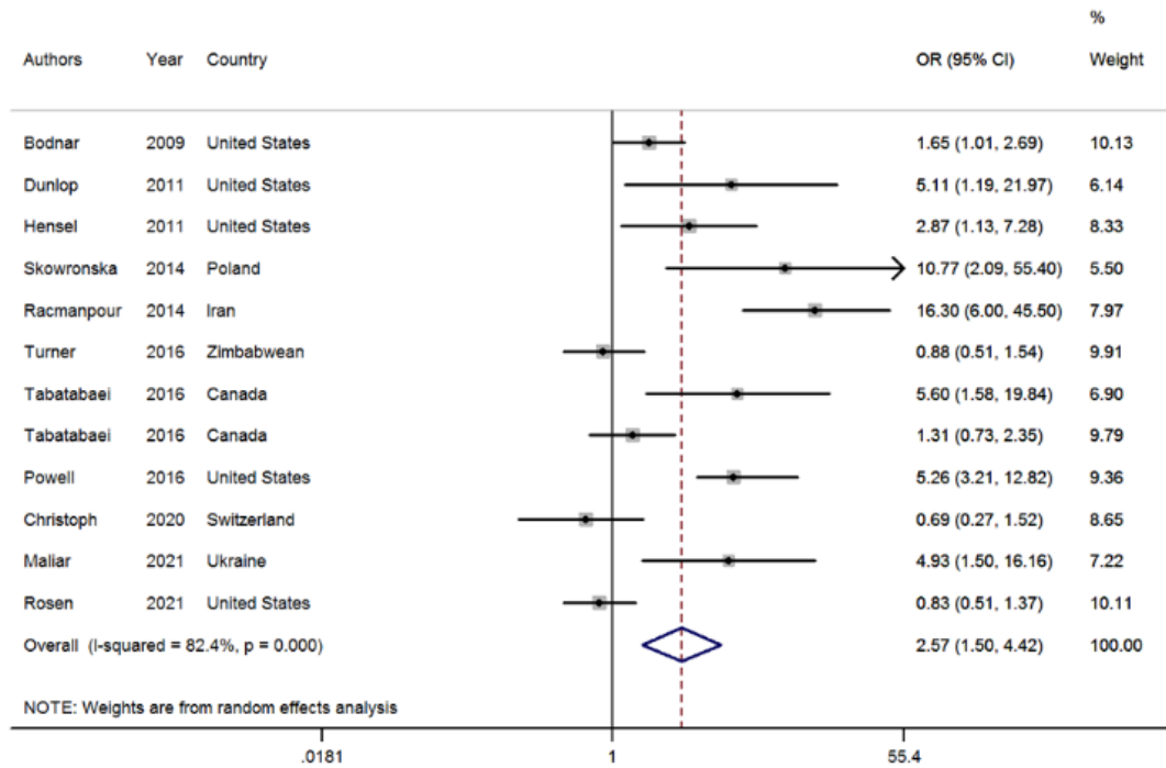
Supplementary Figure 2 Forest plot after removing the first two high-weight studies which considerably influencing the combined effect size. OR, odds ratio; CI, confidence interval. The size of the grey box is positively proportional to the weight assigned to each study, which is inversely proportional to the SE of the OR. The horizontal lines represent the 95% CI.
