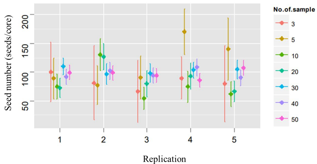
Figure S2 Standard error (SE) of several samples generated randomly from data in Freshwater Bay (FB). Number of samples was from 3 to 50, while the data in FB in May consisted of 60 sample cores. Five-time replication was conducted at each number of samples.
