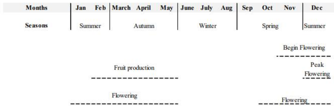
Figure S1 Annual cycle of sexual reproduction of H. ovalis in Swan-Canning estuary (Kilminster and Forbes 2014)
