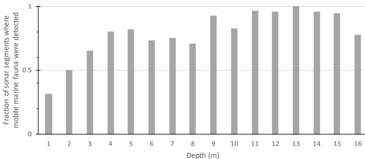
Supplementary Figure S1. Bar plot of overall mobile marine fauna presence in sonar segments by water depth.
