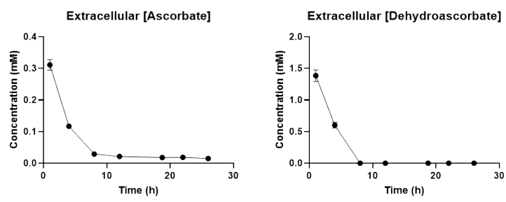
Supplementary Figure 5: Ascorbate and dehydroascorbate concentrations in the growth medium during B. pertussis Tohama I culture. Concentrations of metabolites (mM) were monitored by NMR.
