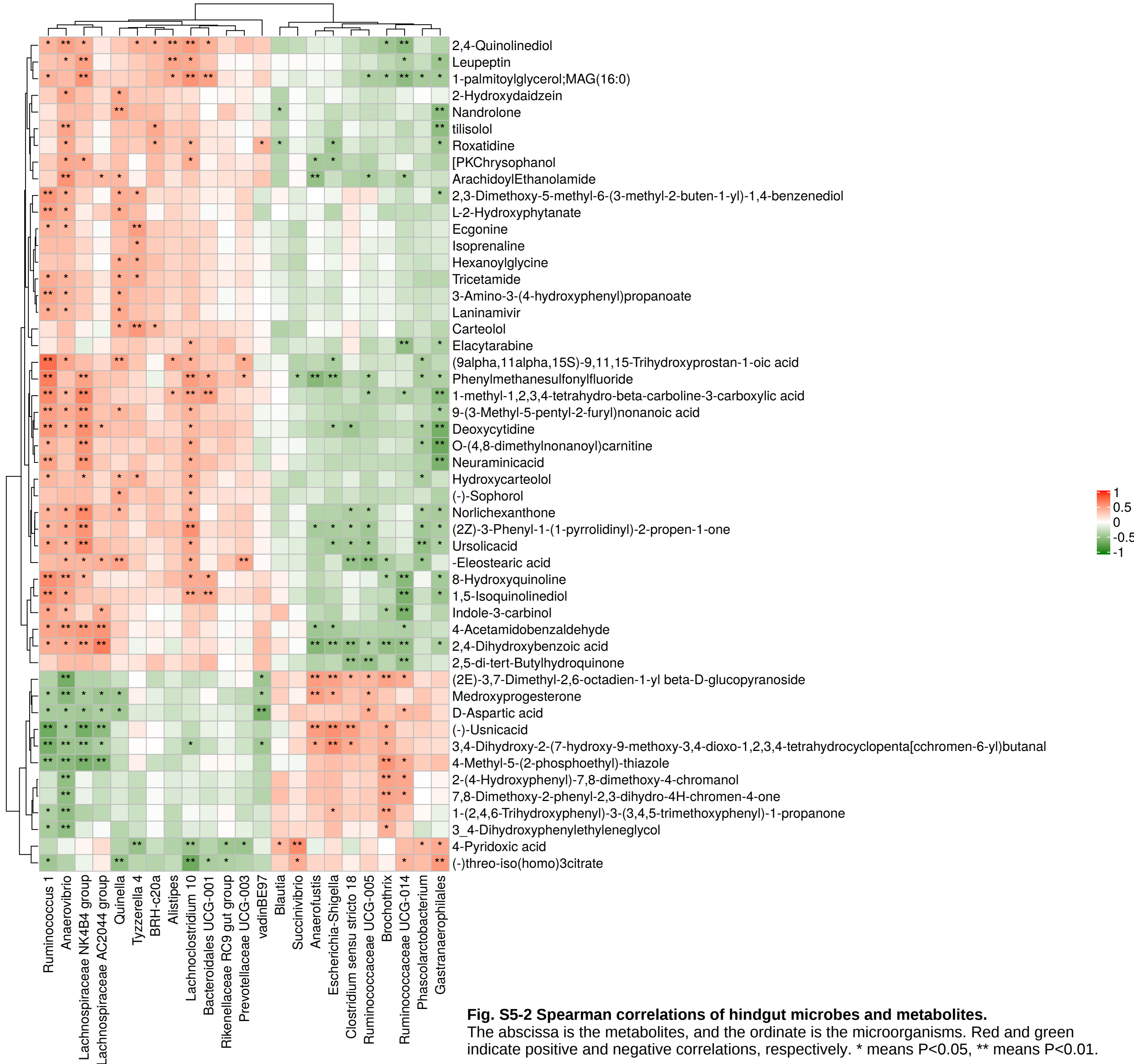
Correlation heatmap
