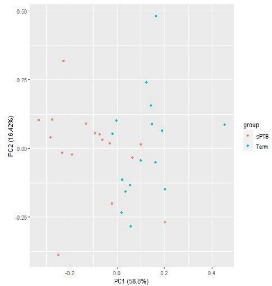
Figure S1. PCA analysis of 5 circadian lincRNAs to visualize the clusters due to the differences in 5 circadian lincRNAs between sPTB and term births and the corresponding variability. A is for GSE73712 and B for GSE174415.
