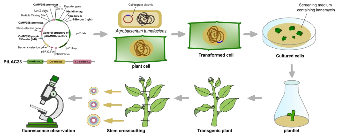
Fig. S1 Schematic diagram of experimental process of agrobacterium-mediated transformation (ATMT), transgenic plant screening, freehand section and fluorescence observation.
