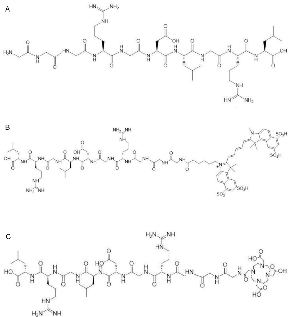
Figure S1. The structure of (A) peptide G2-SFLAP3, (B) G2-SFLAP3-Cy5.5, and (C) DOTA-G2-SFLAP3.
