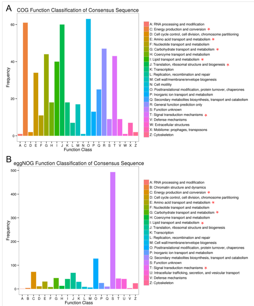
Supplementary Figure 4. DEG direct homology classification according to (A) CGO classification; (B) eggNOG classification.
