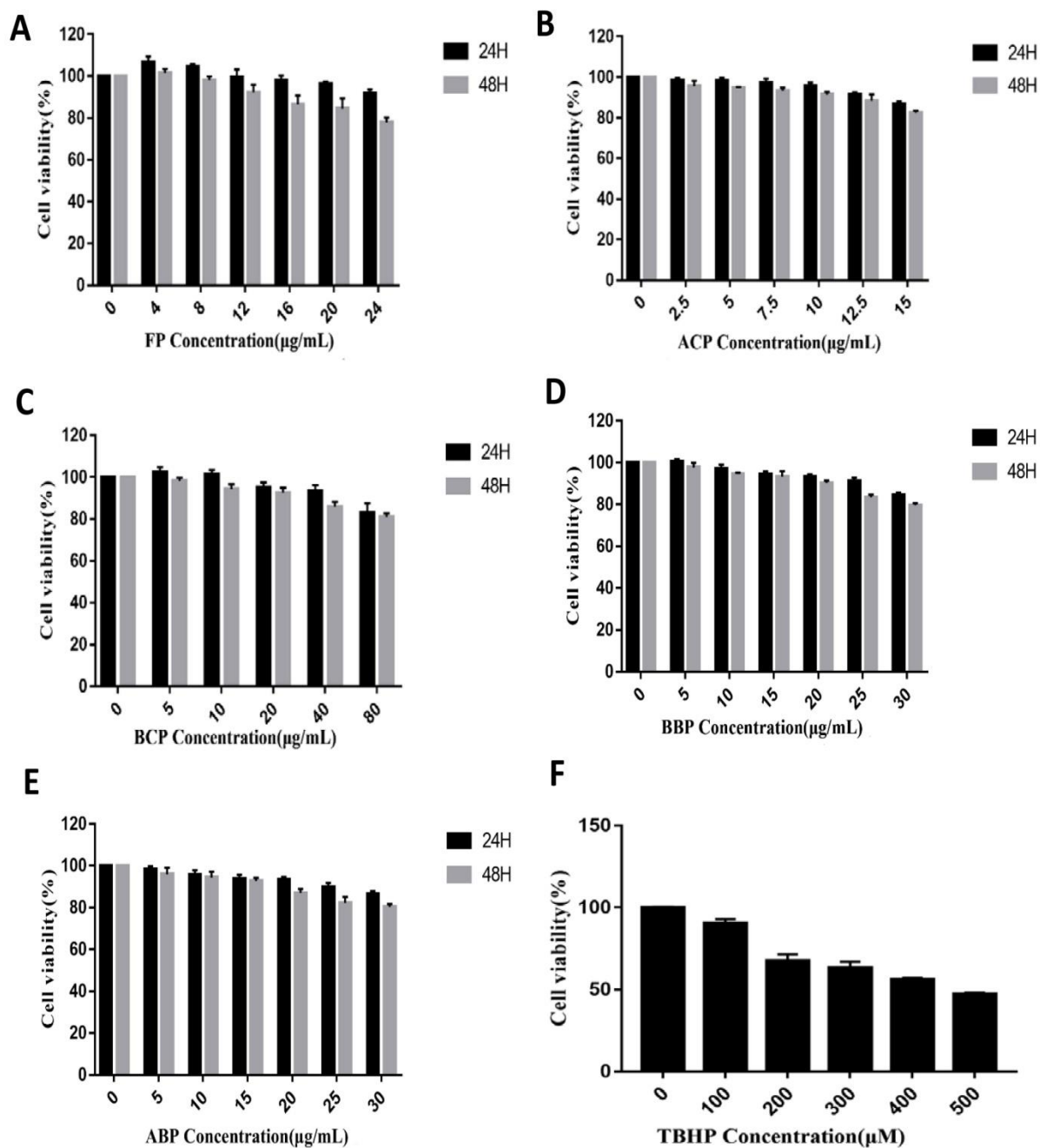
Figure S1 Evaluation of HUVEC viability using MTT assay after exposure to different concentrations of phenolics for 24 h or 48h and different concentrations of TBHP for 24 h, FP (A), ACP (B), BCP (C), BBP (D), ABP (E), TBHP (F).
