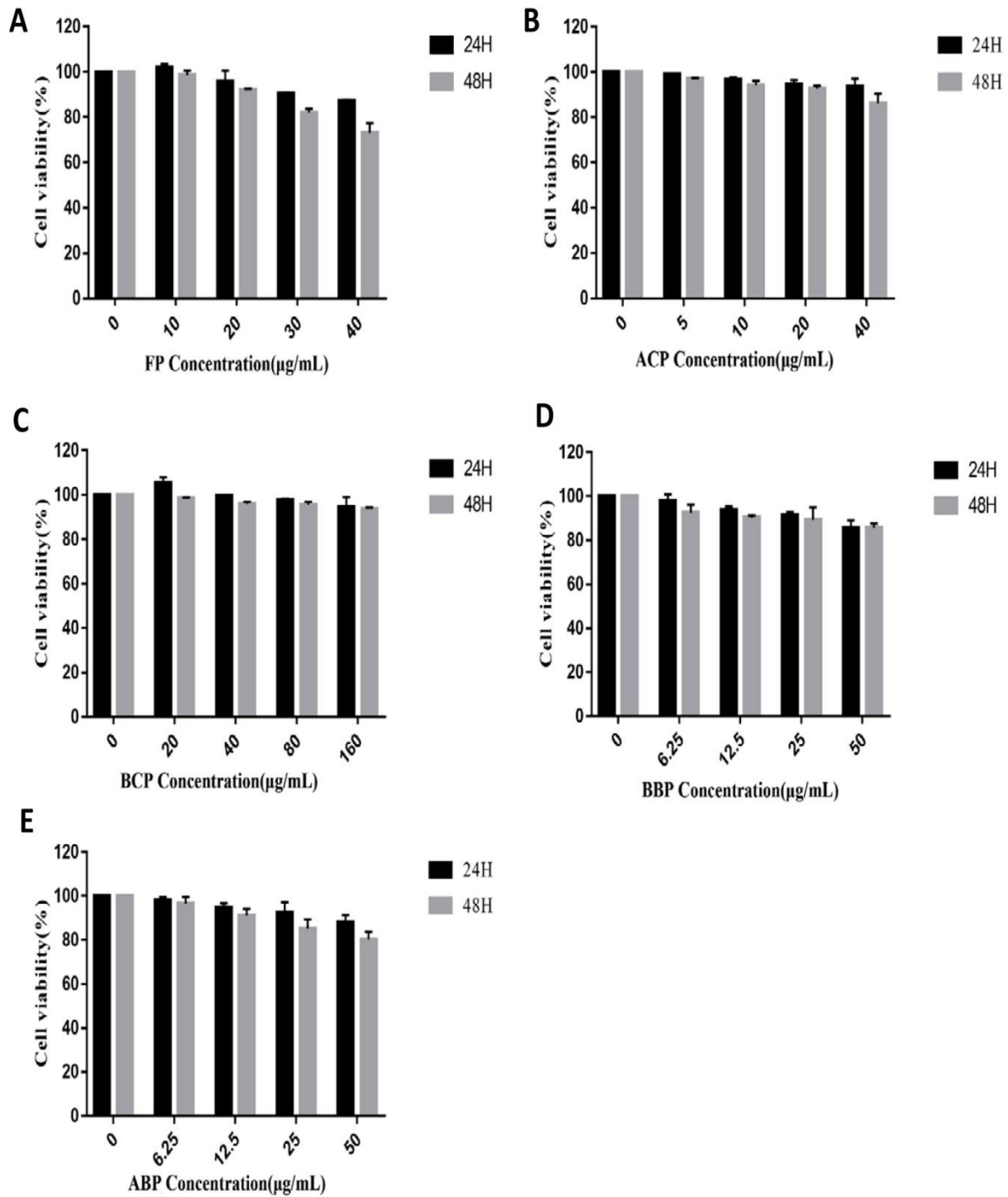
Figure S2 Evaluation of RAW264.7 viability using MTT assay after exposure to different concentrations of phenolics for 24 h or 48h, FP (A), ACP (B), BCP (C), BBP (D), ABP (E).
