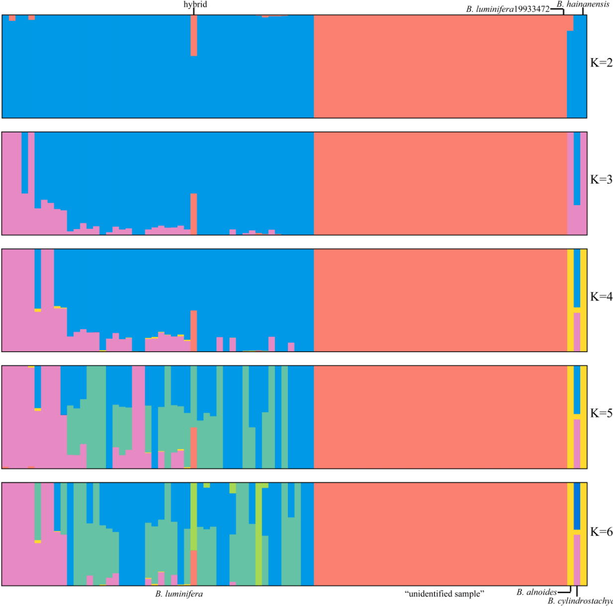
Figure S1 Admixture results at K values from 2 to 6 based on 40,209 SNPs.
