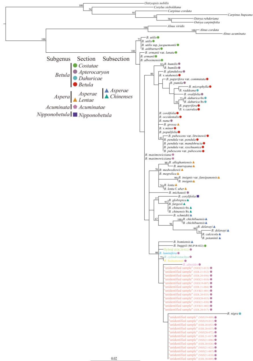
Figure S5 Phylogenetic tree from the maximum-likelihood analysis of the “unidentified sample” using ITS sequences.
