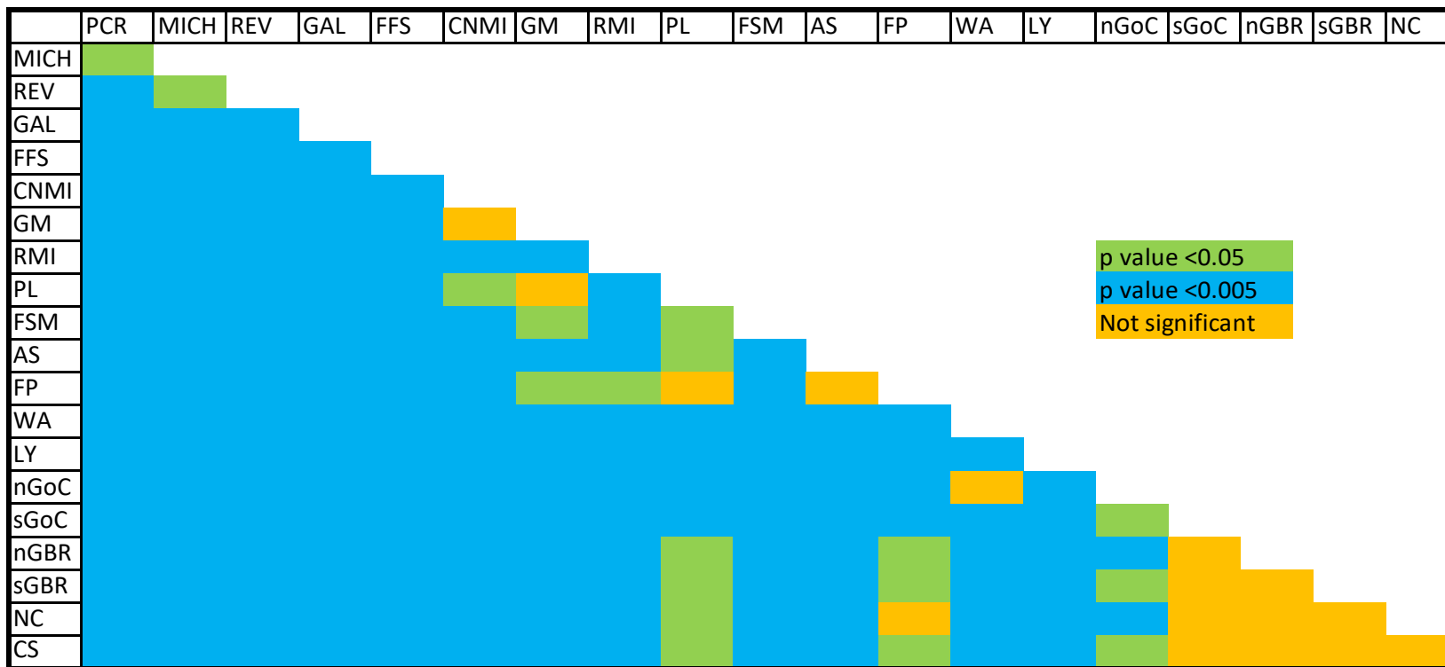
Supplementary Figure 2. Results of pairwise FST tests (6 loci) (Blue, p < 0.005 ; green, p < 0.05 ; orange, p > 0.05 ) PCR = Guanacaste, Costa Rica; MICH = Playa Colola, Michoacán, Mexico; REV = Islas Revillagigedo, Mexico; GAL = Galapagos Islands, Ecuador; FFS = French Frigate Shoals, Hawaii, USA; CNMI = Commonwealth of the Northern Mariana Islands, USA; GM = Guam, USA; RMI = Republic of the Marshall Islands; PL = Palau; WAN = Wan-an Island, Taiwan; LY = Lanyu Island, Taiwan; FSM = Federated States of Micronesia; AS = American Samoa, USA; FP = French Polynesia; nGoC = northern Gulf of Carpentaria, Northern Territory, Australia; sGoC = southern Gulf of Carpentaria, Queensland Australia; CS = Coral Sea Islands, Australia; sGBR = Southern Great Barrier Reef, Australia; nGBR = Northern Great Barrier Reef, Australia; NC = New Caledonia
