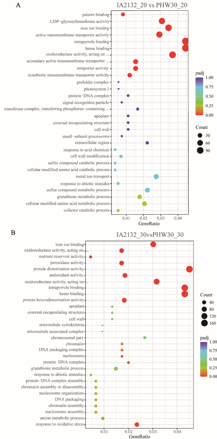
Supplementary Figure 3. GO analysis. (A) Enriched GO terms at the 20 th day after pollination. In the figure, the abscissa is the ratio of the number of differentially annotated genes on GO Term to the total number of differentially annotated genes on GO Term; the vertical axis is GO Term (first 30); the size of dots represents the number of genes annotated on GO term; the color from red to purple represents the significance of enrichment, the same as below. (B) GO terms at the 30 th day after pollination.
