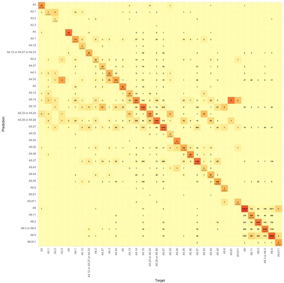
Figure S6 – Confusion matrix for model M36
