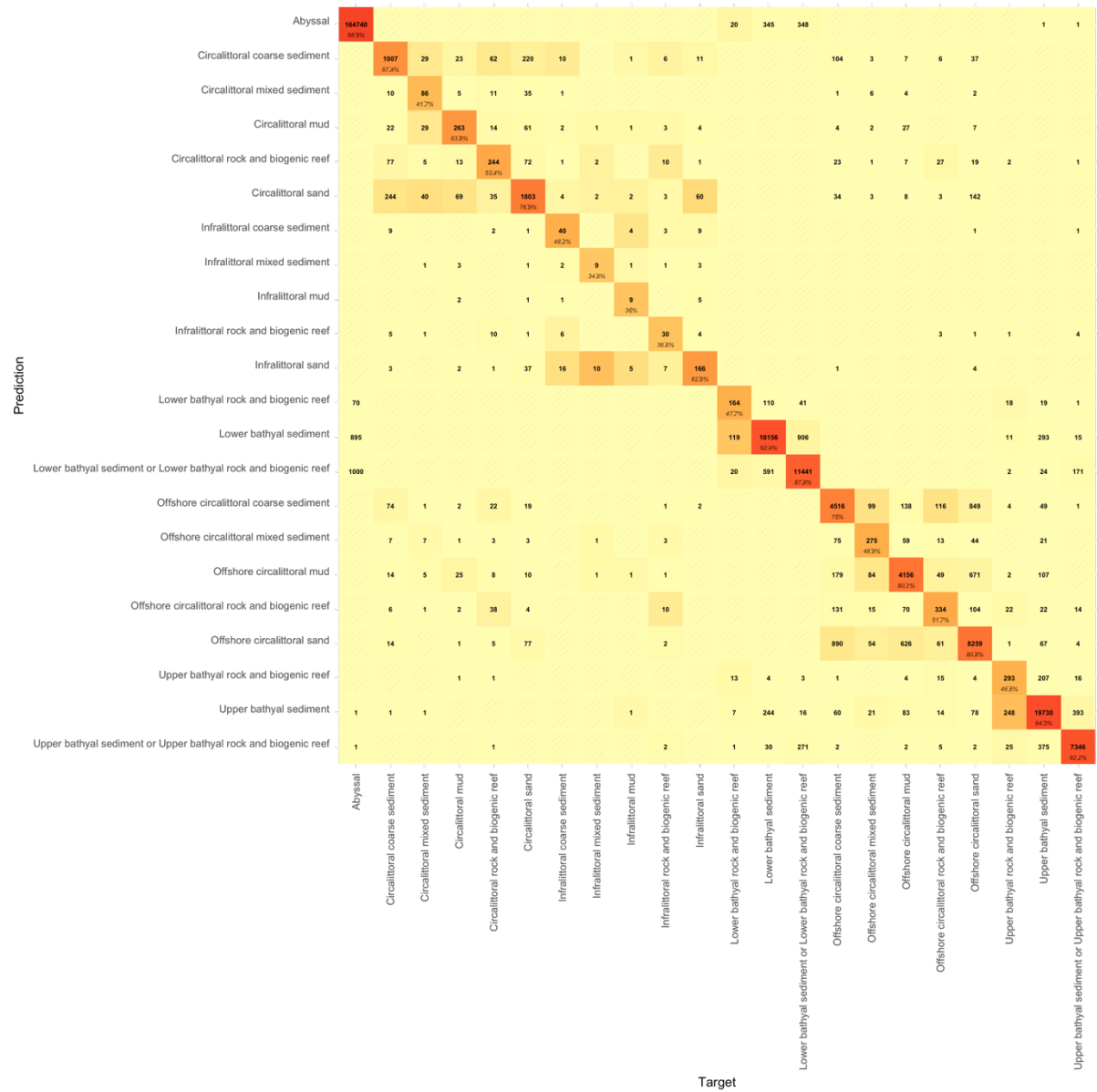
Figure S7 – Confusion matrix for model M37
