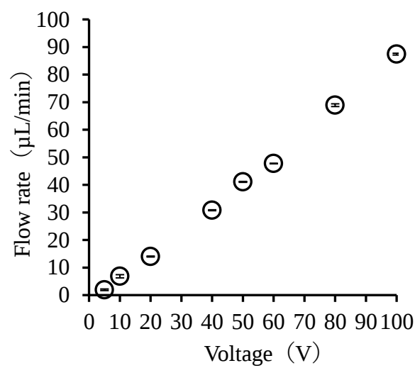
Supplemental Figure 1. The relationship between applied voltage and flow rate. Each point shows the mean \pm S.D. (n = 5).
