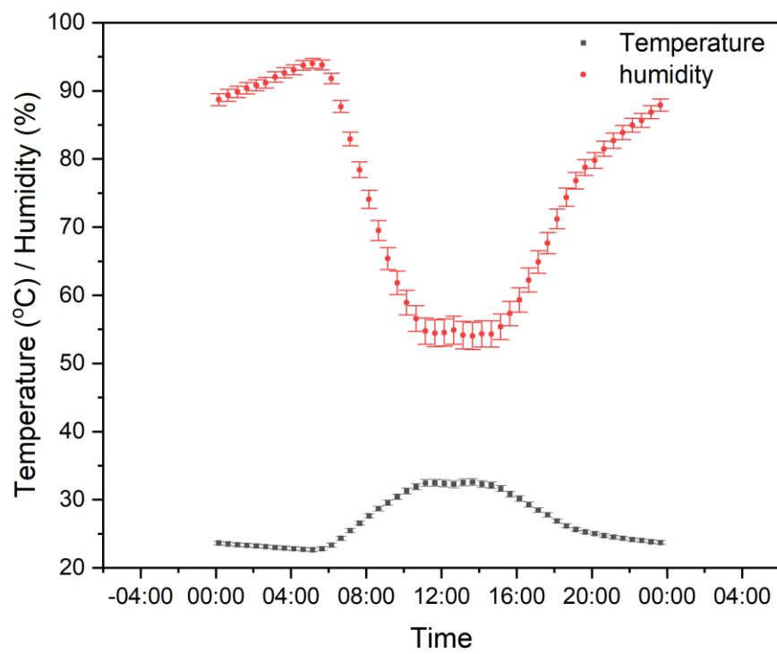
Figure S2 Typical diurnal pattern of temperature and humidity in the experimental period.
