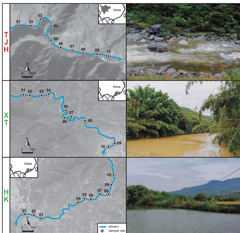
Figure S1. The study areas of this study: Tangjiahe National Nature Reserve (TJH), Xintian town (XT), and Hekou town (HK). Environmental DNA sampling maps (left side) show the rivers (blue lines) and locations of the eDNA sampling sites (black dots). The natural environment of each river is shown on the right.
