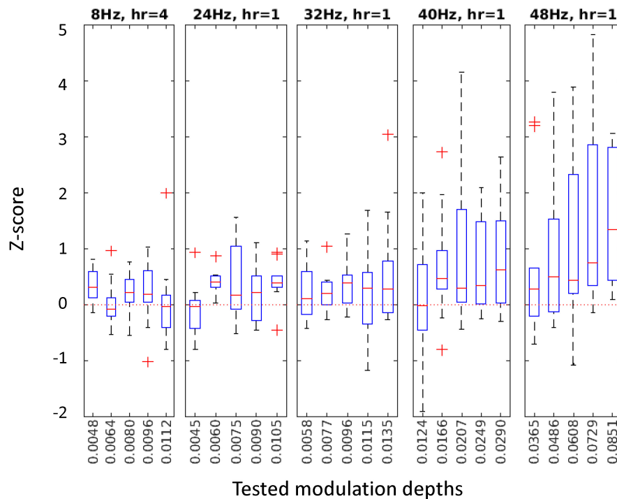
Figure S1. z-score distributions at the best harmonic component for each condition in Experiment 1. Different frequencies with their selected harmonic component in separate panels, tested MDs on the horizontal axes.
