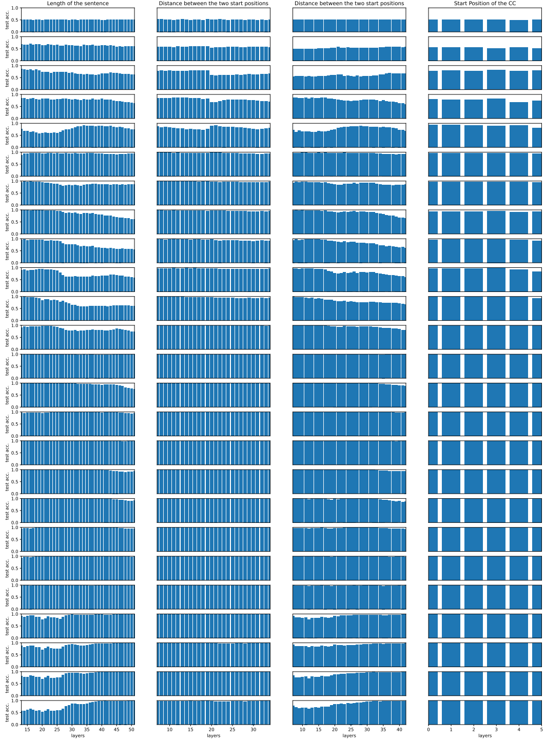
Figure A1: Full results for BERT LARGE on artificial data. Columns indicate the variable that the training and test set controls for.
