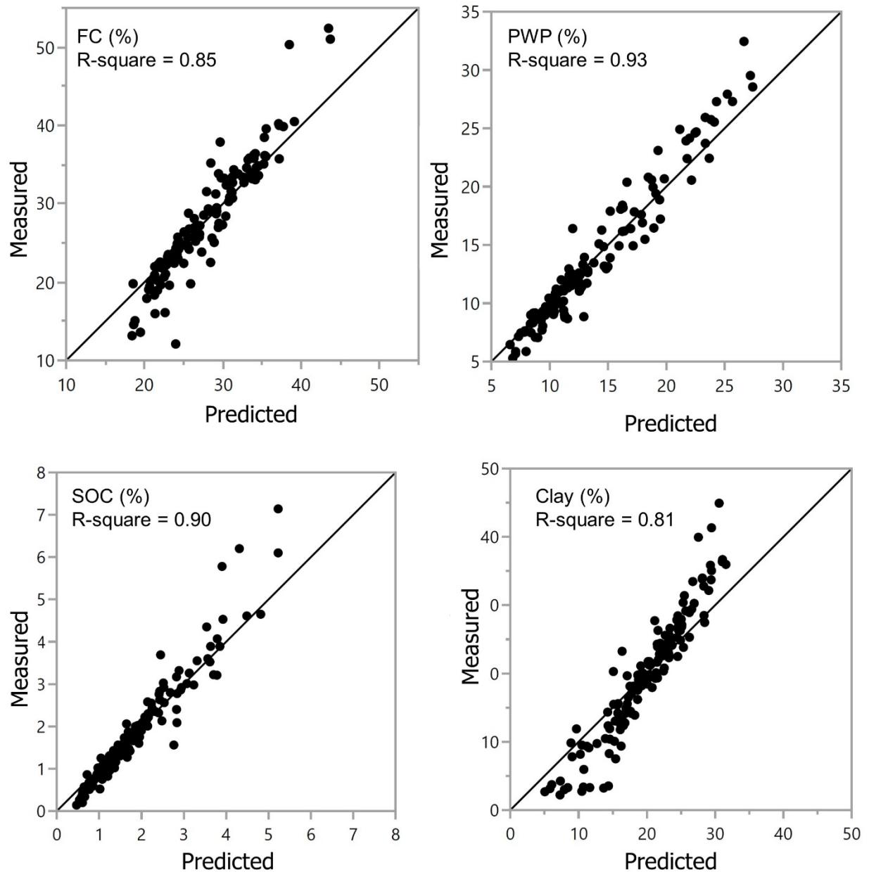
Supplementary Figure S1. Scatter plots for predicted and measured values obtained from calibrations using mid-infrared (MIR) spectroscopy coupled with random forest (RF) regression for field capacity –33 kPa (FC), permanent wilting point –1500 kPa (PWP), soil organic carbon (SOC) and clay
