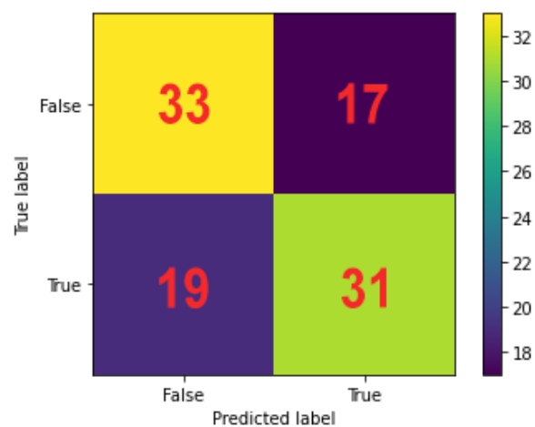
Figure 9. Model C Confusion Matrices using Fake image Dataset
