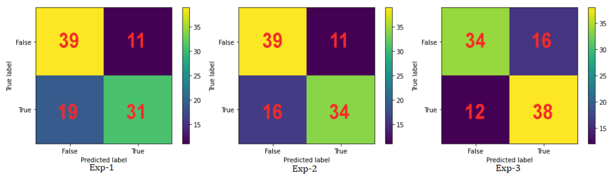
Figure 7. Model A Confusion Matrices using Fake Image Dataset
