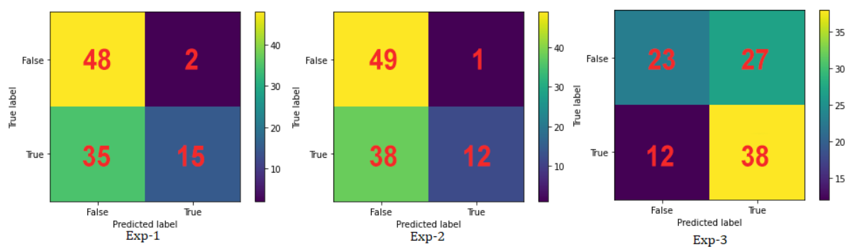
Figure 8. Model B Confusion Matrices using Fake Image Dataset
