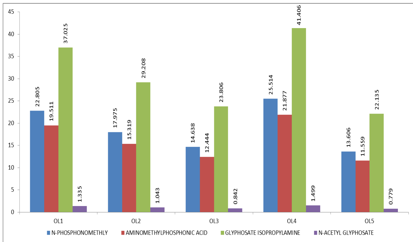
Figure 1. Residues concentrations (mg/L) of Glyphosate and its metabolites present in the livers of Catfish offered for sale in Ojoo Fish Market
