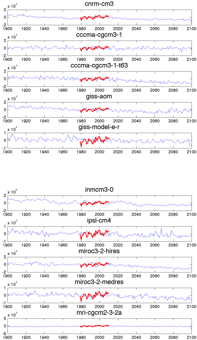
Figure A1. Comparison of Ross Sea sea ice extent values derived from satellite observations (red line) and Ross Sea sea ice values derived from the AOGCMs.
