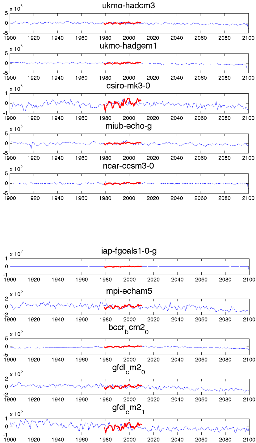
Figure A2. Comparison of Ross Sea sea ice extent values derived from satellite observations (red line) and Ross Sea sea ice values derived from the AOGCMs.
