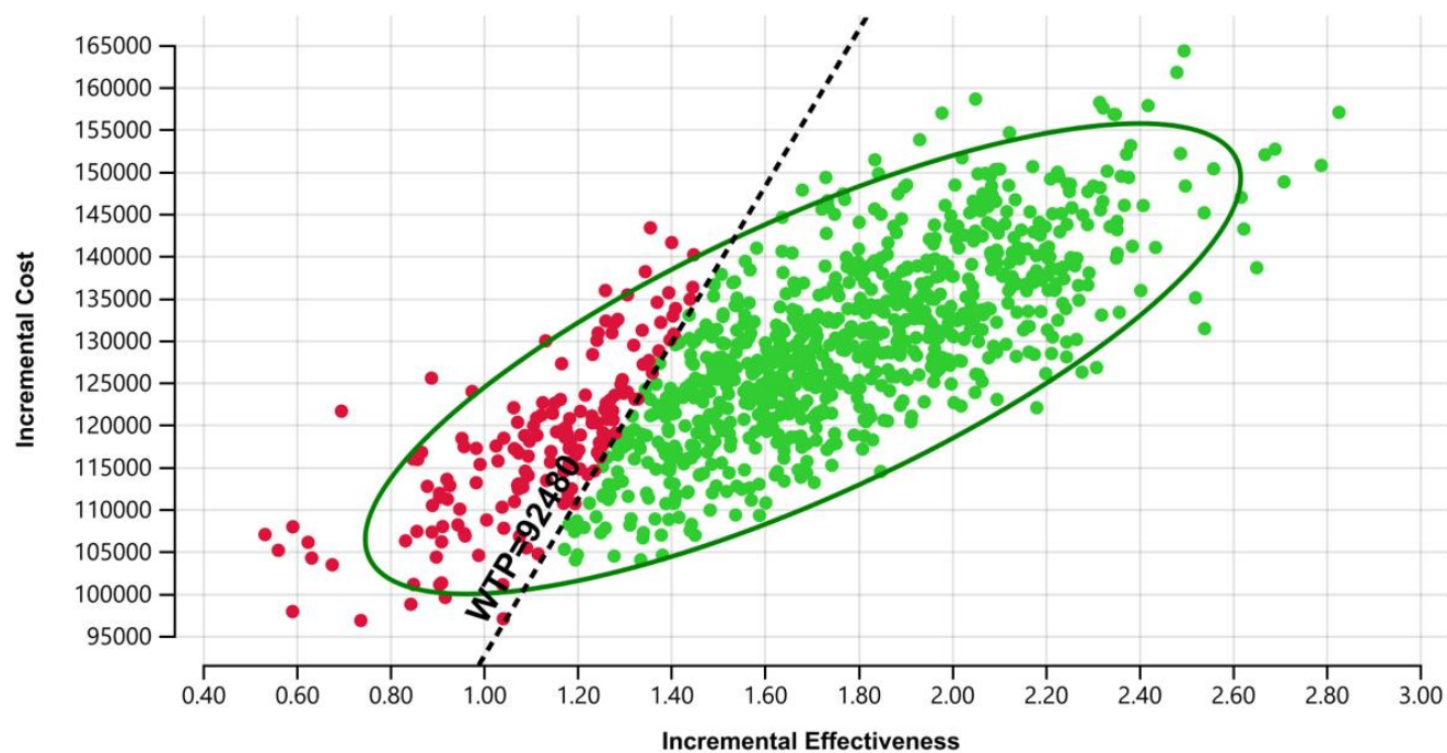
Appendix Figure 1: Incremental cost-effectiveness scatterplot of atezo-bev versus sorafenib. WTP, Willingness to pay
