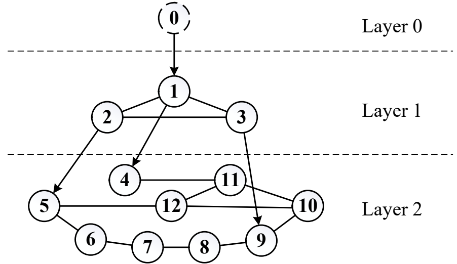
(b) Reconfigured system topology
