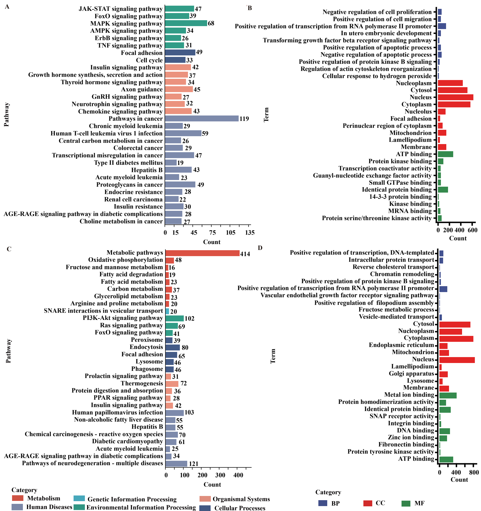
Figure S5. The enrichments of DE lncRNAs in Min resistance (MR) vs. Min control (MC) groups. (A) KEGG pathway enriched by DE lncRNAs with significant up-regulation expression in MR vs. MC. (B) GO entries enriched by DE lncRNAs with significant up-regulation expression in MR vs. MC. (C) KEGG pathway enriched by DE lncRNAs with strong down-regulation expression in MR vs. MC. (D) GO entries enriched by DE lncRNAs with strong down-regulation expression in MR vs. MC.
