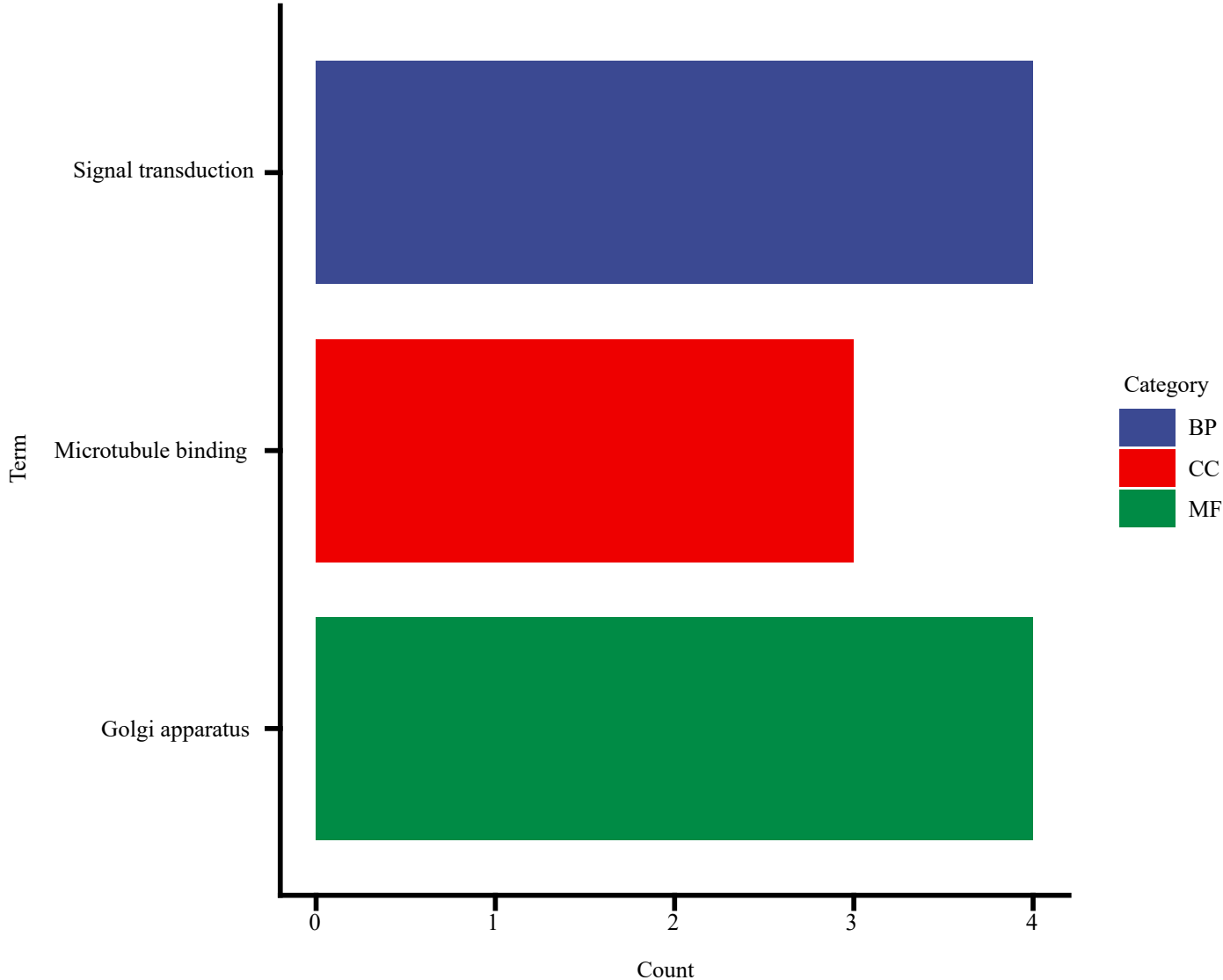
Figure S8. The enrichments of DE miRNAs in Min dead (MD) vs. Min resistance (MR) groups. GO entries enriched by DE miRNAs with strong down-regulation expression in MD vs. MR.
