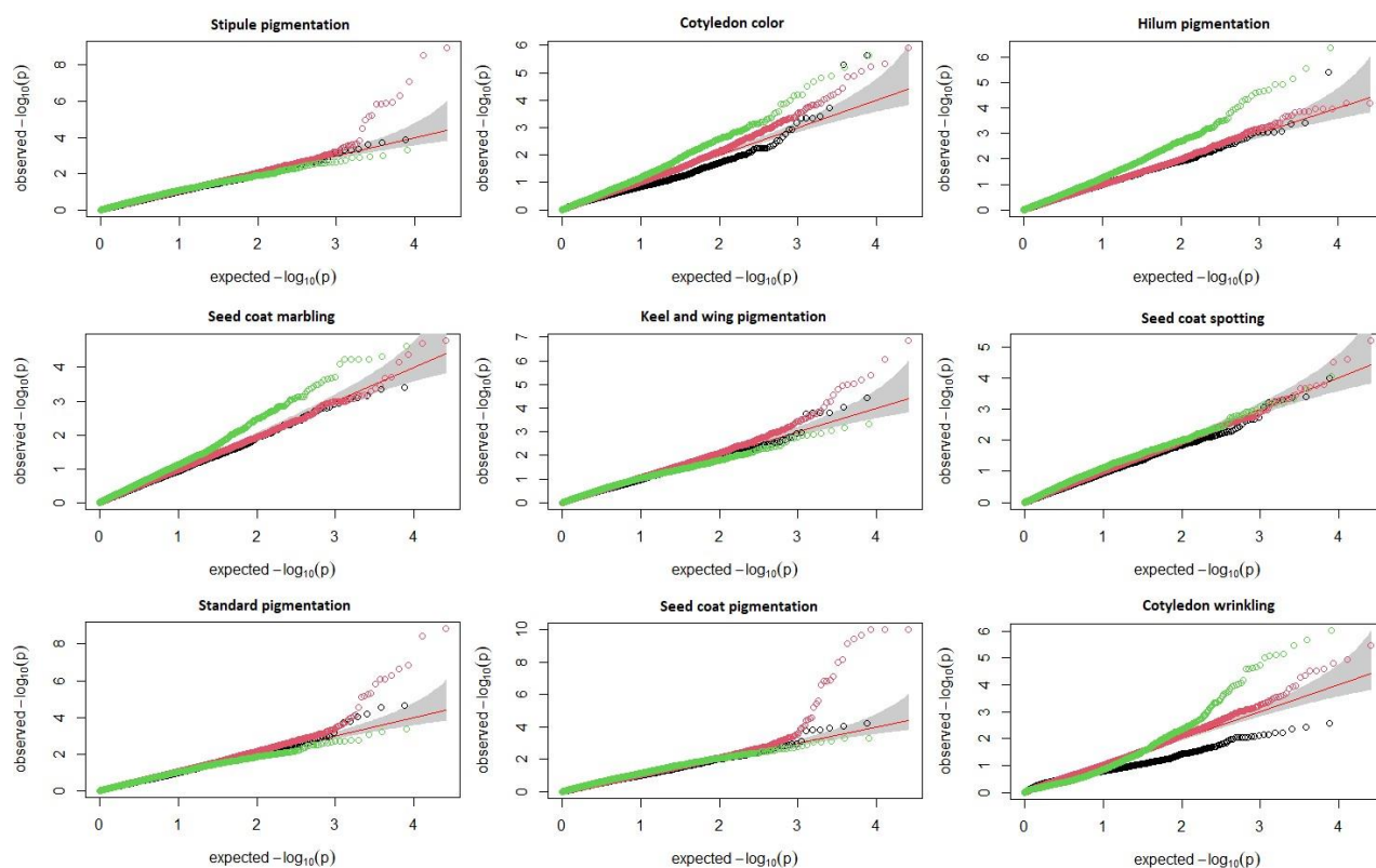
Supplementary Figure 1. Quantile-Quantile plots of expected vs. observed association scores of 41,114 SNPs for nine qualitative traits. Different colors were attributed to SNPs basing on a classification in three categories depending on the ratio of SNP expected variances in different population strata (Milet et al., 2020), which were defined by DAPC cluster membership. The red line represents equality between the expected and observed quantiles and the grey area the associated 95% confidence interval.
