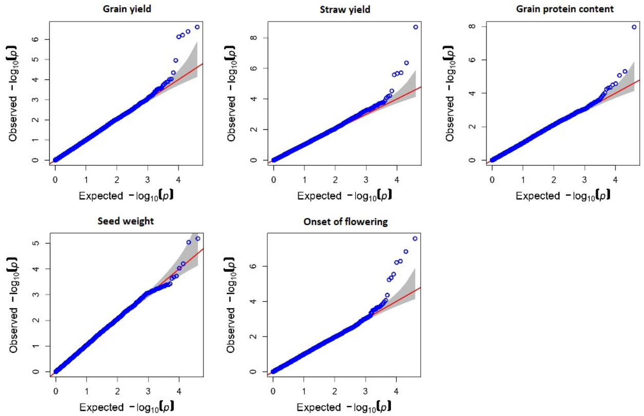
Supplementary Figure 2. Quantile-Quantile plots of expected vs. observed association scores of 41,114 SNPs for five quantitative traits. The red line represents equality between the expected and observed quantiles and the grey area the associated 95% confidence interval.
