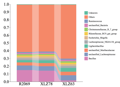
Seed:Genus level
