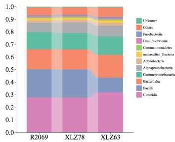
Seed:Class level
