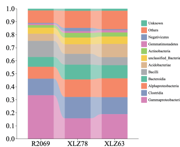
Seed-P:Class level
