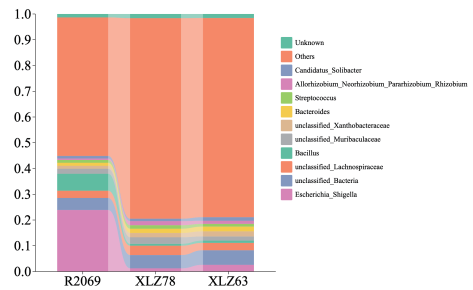
Seed-P:Genus level
