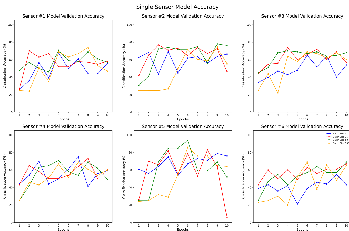
Figure S1. Classification accuracy of models trained on data from a single sensor
