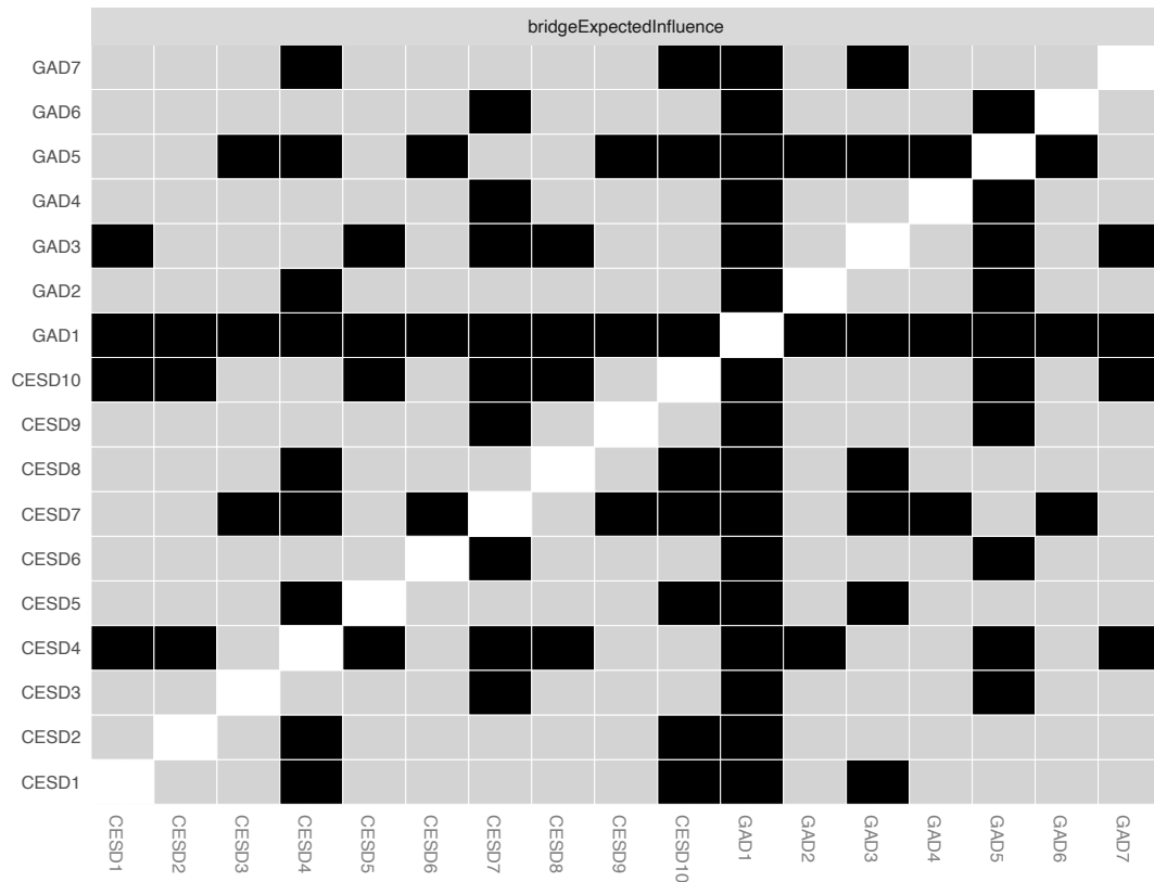
Supplementary Figure 4 Bootstrapped difference test for node bridge expected influences in the network
