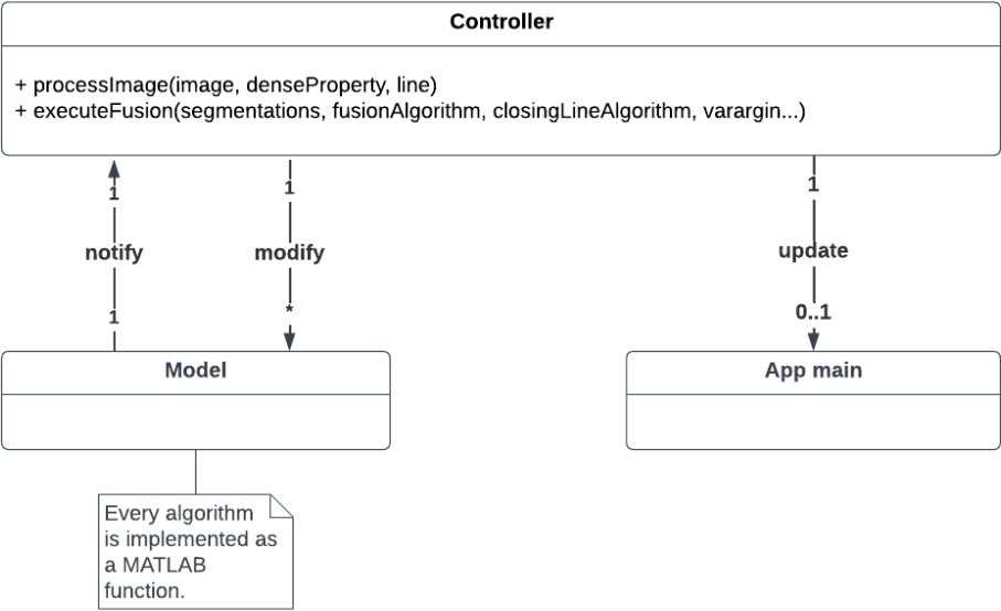
Supplementary Figure 1.1: TDSFT MVC architecture.
