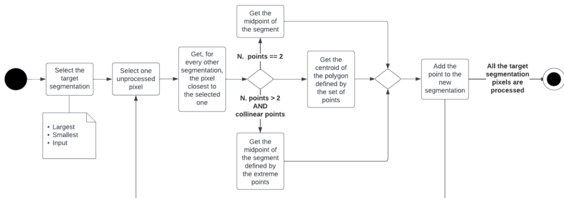
Supplementary Figure 2.4: Flowchart of “ Average With Target ” algorithms.
