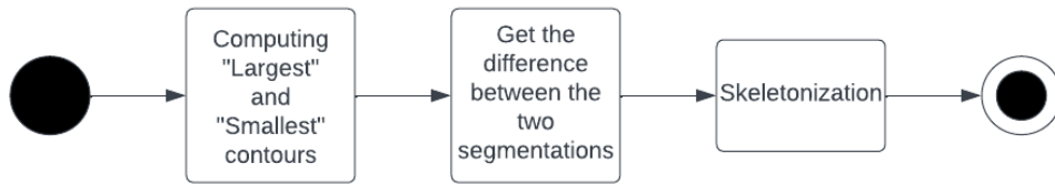
Supplementary Figure 2.3: Flowchart of “ Average Smallest And Largest ” algorithm.
