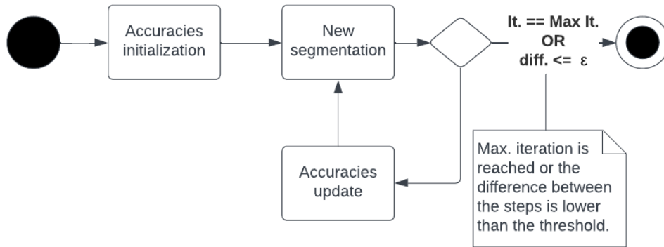
Supplementary Figure 2.6: Flowchart of “ STAPLE ” algorithm.
