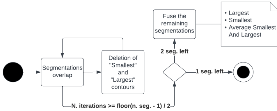
Supplementary Figure 2.5: Flowchart of “ Middle ” algorithm.
