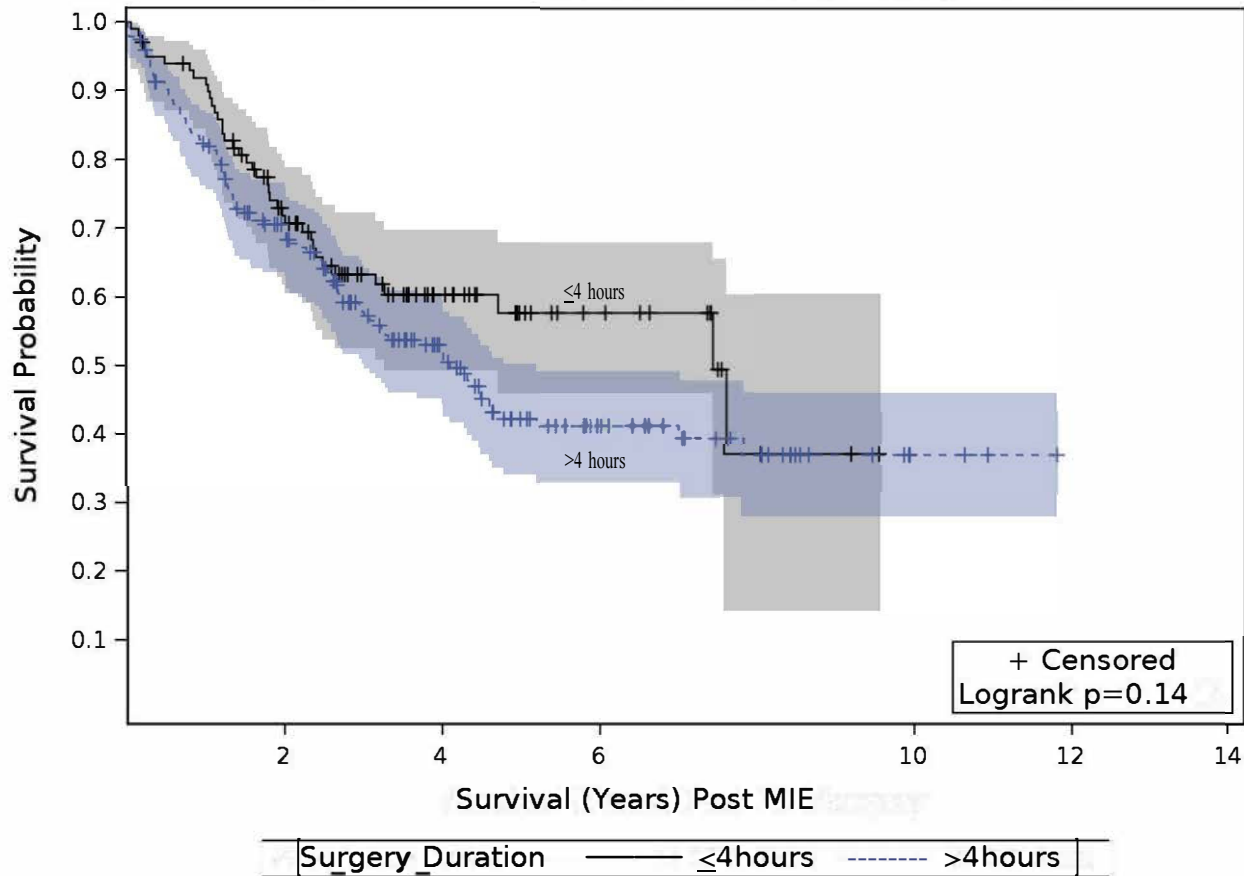
Kaplan-Meier MIE Survival Estimates by Surgery Duration
