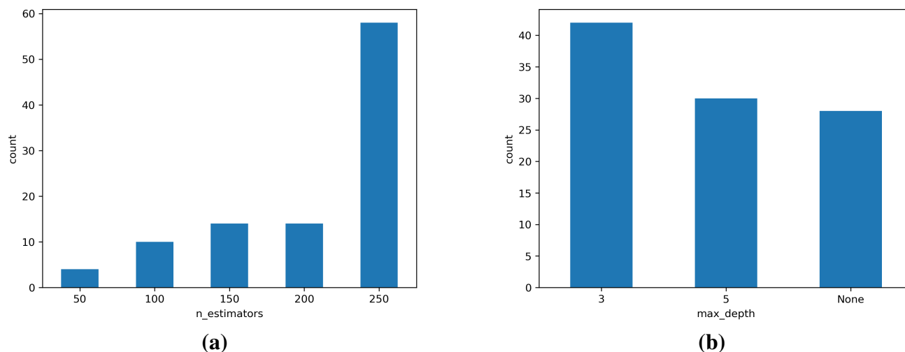
Figure S2: Stability analysis of tuned parameters in nested cross-validation for RF: (a) n_estimators (b) max_depth.
