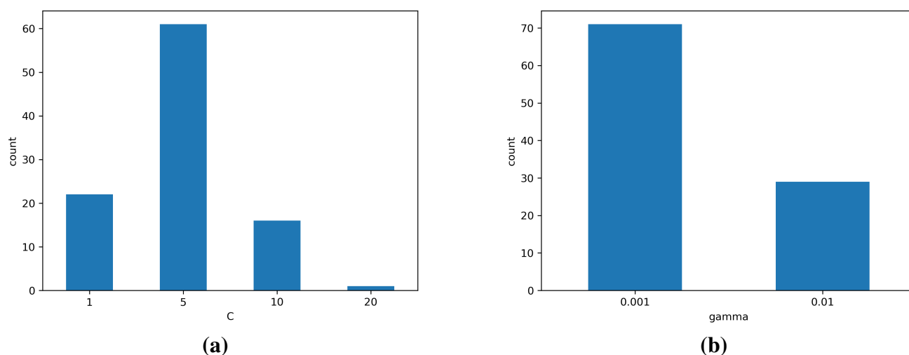
Figure S4: Stability analysis of tuned parameters in nested cross-validation for SVM: (a) C (b) gamma .
