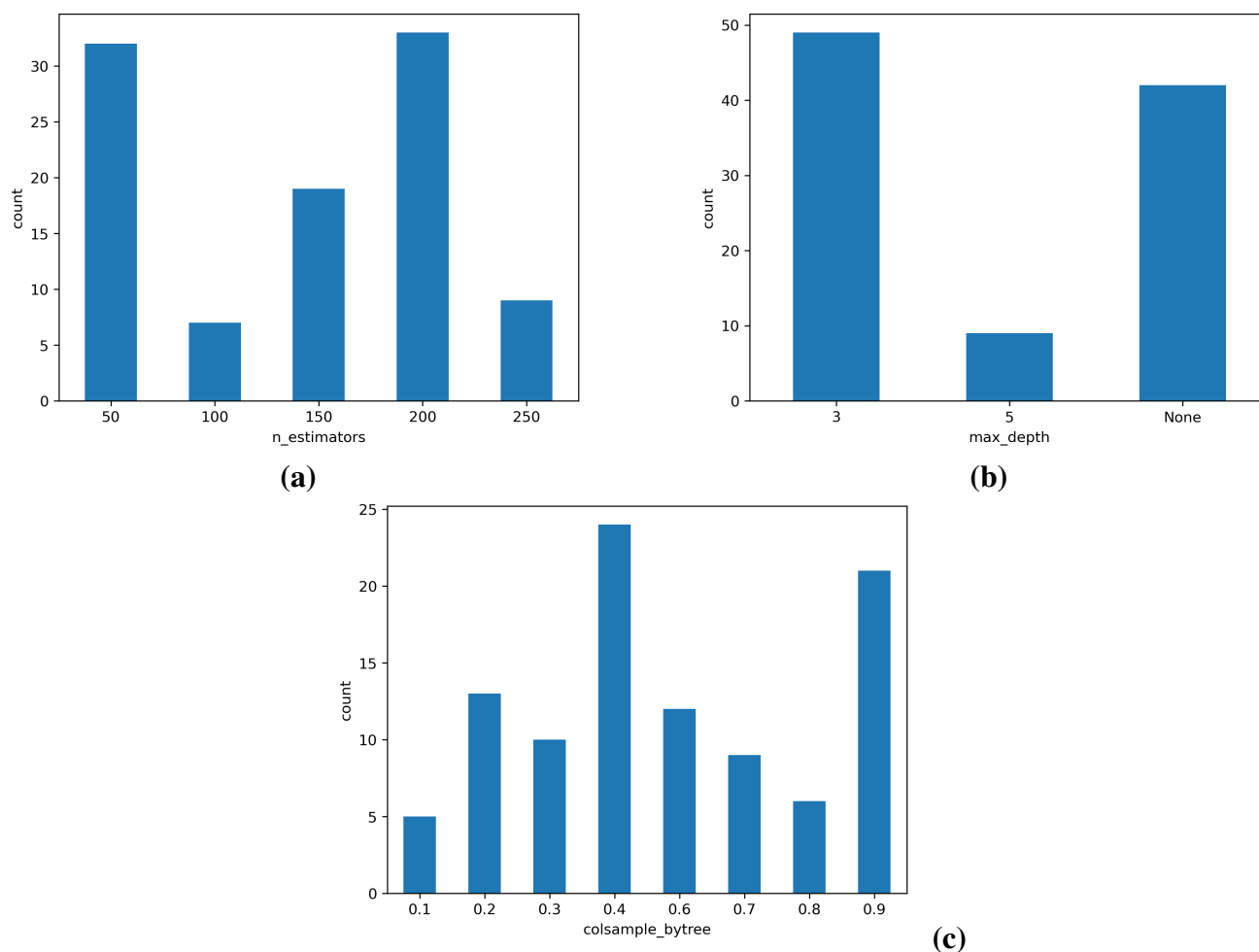
Figure S3: Stability analysis of tuned parameters in nested cross-validation for XGBoost: (a) n_estimators (b) max_depth (c) colsample_bytree .
