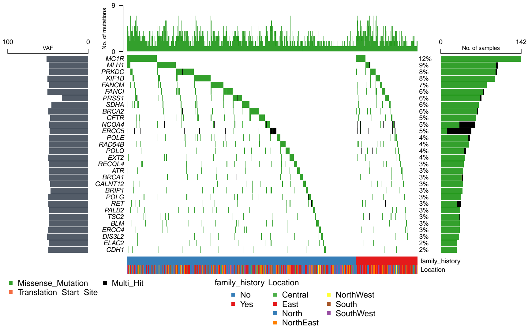
Figure S3. Mutations spectrum of genes with high-frequency deleterious mutation
