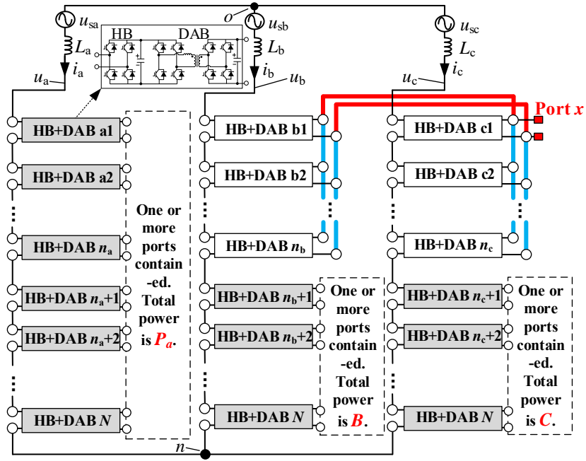
Figure A3. The IDBS-MPET containing D-Port in phase b and phase c.
