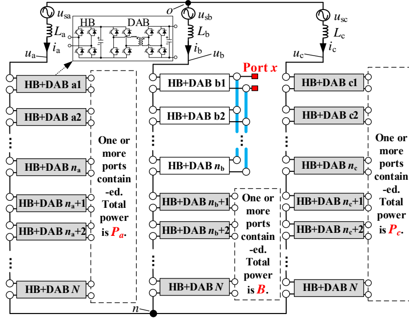
Figure A1. The IDBS-MPET containing S-Port in phase b.
