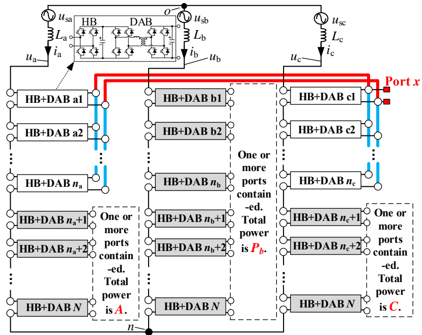
Figure A4. The IDBS-MPET containing D-Port in phase a and phase c.
