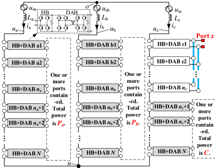
Figure A2. The IDBS-MPET containing S-Port in phase c.
