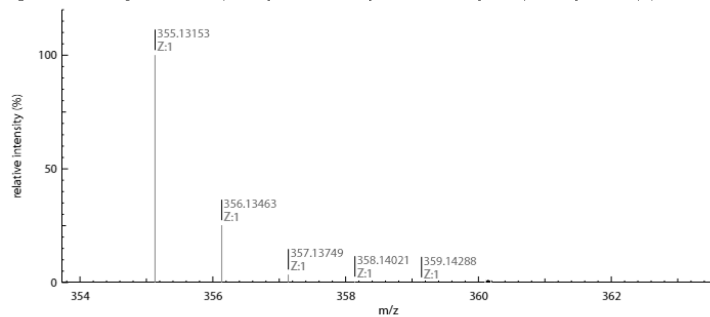
Figure S27: Mass spectrum of N'-(1-benzyl-2-oxo-1,2-dihydro-3H-indol-3-ylidene)benzohydrazide (5i):
