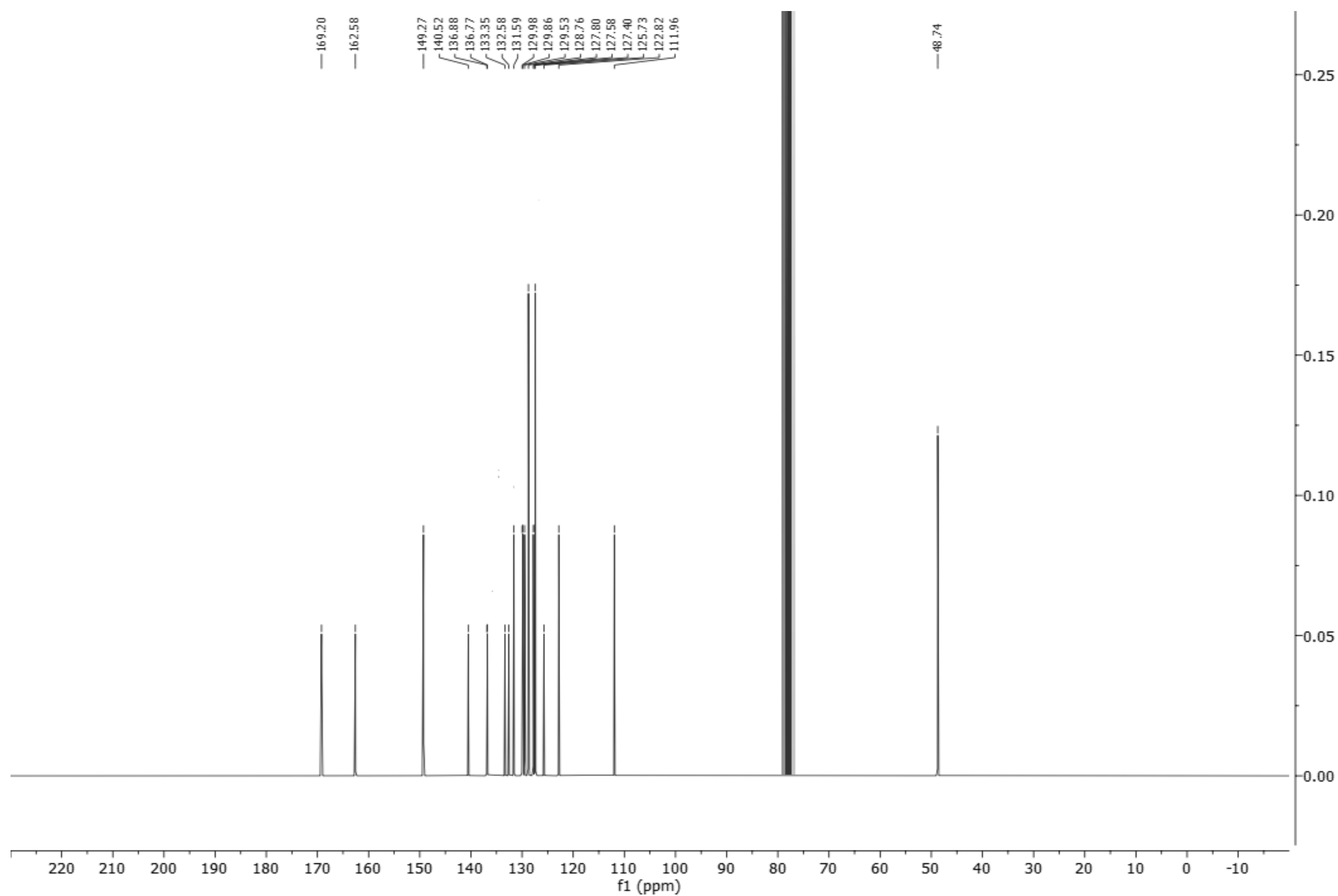
Figure S15: ^{13}\text{C} NMR spectrum of N'-(1-benzyl-2-oxo-1,2-dihydro-3H-indol-3-ylidene)-2-chlorobenzohydrazide (5h):
