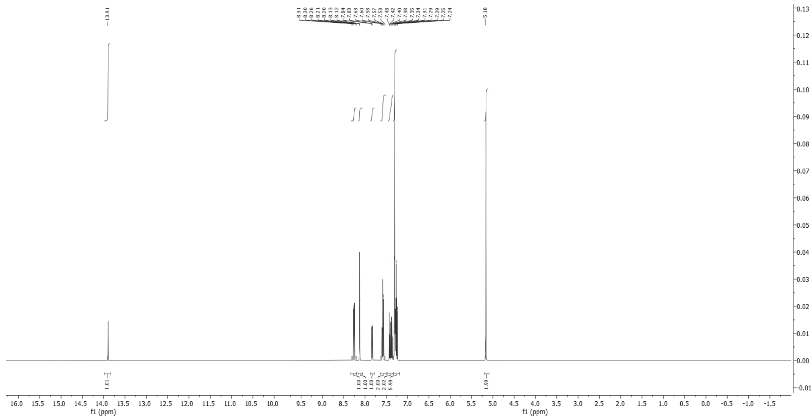
Figure S6: ^1\text{H} NMR spectrum of N'-(1-benzyl-2-oxo-1,2-dihydro-3H-indol-3-ylidene)-3-iodobenzohydrazide (5c)
