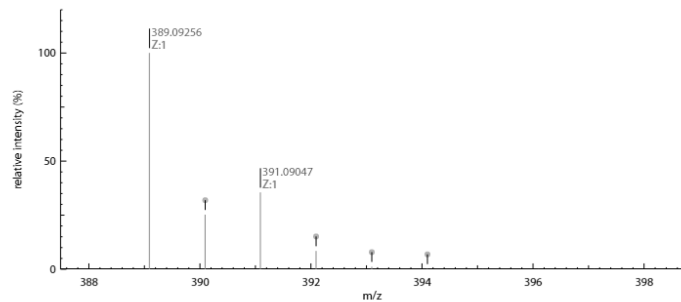
Figure S26: Mass spectrum of N'-(1-benzyl-2-oxo-1,2-dihydro-3H-indol-3-ylidene)-2-chlorobenzohydrazide (5h):
