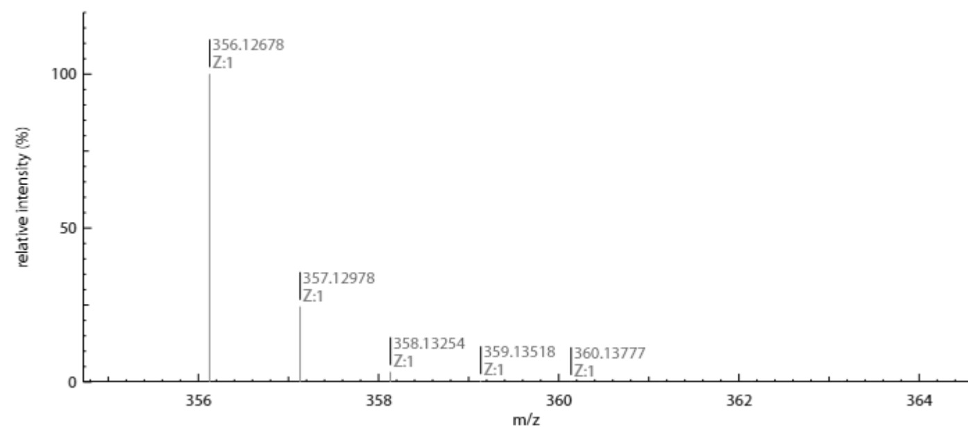
Figure S24: Mass spectrum of N'-(1-benzyl-2-oxo-1,2-dihydro-3H-indol-3-ylidene)pyridine-2-carbohydrazide (5f):
