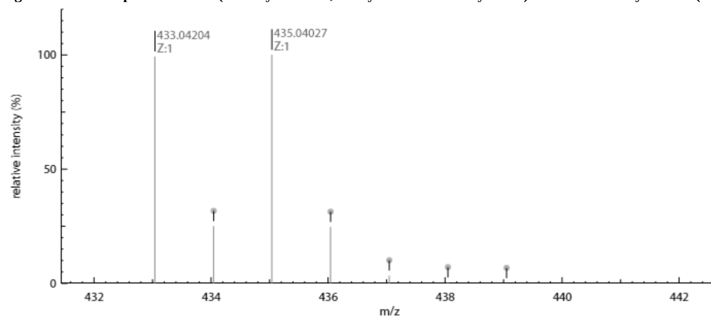
Figure S20: Mass spectrum of N'-(1-benzyl-2-oxo-1,2-dihydro-3H-indol-3-ylidene)-3-bromobenzohydrazide (5b)
