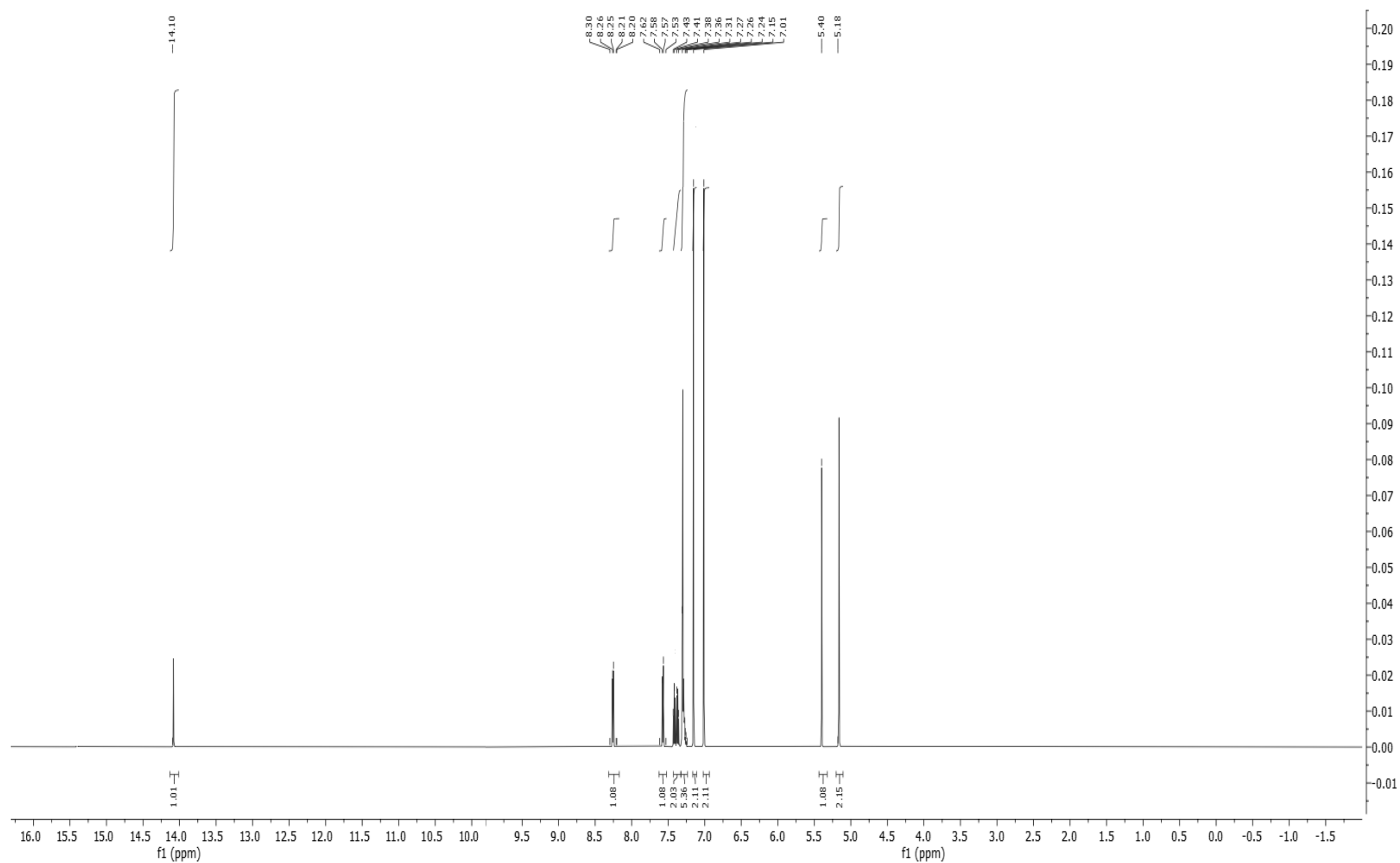
Figure S14: ^1\text{H} NMR spectrum of N'-(1-benzyl-2-oxo-1,2-dihydro-3H-indol-3-ylidene)-3,4,5trihydroxybenzohydrazide (5g):
