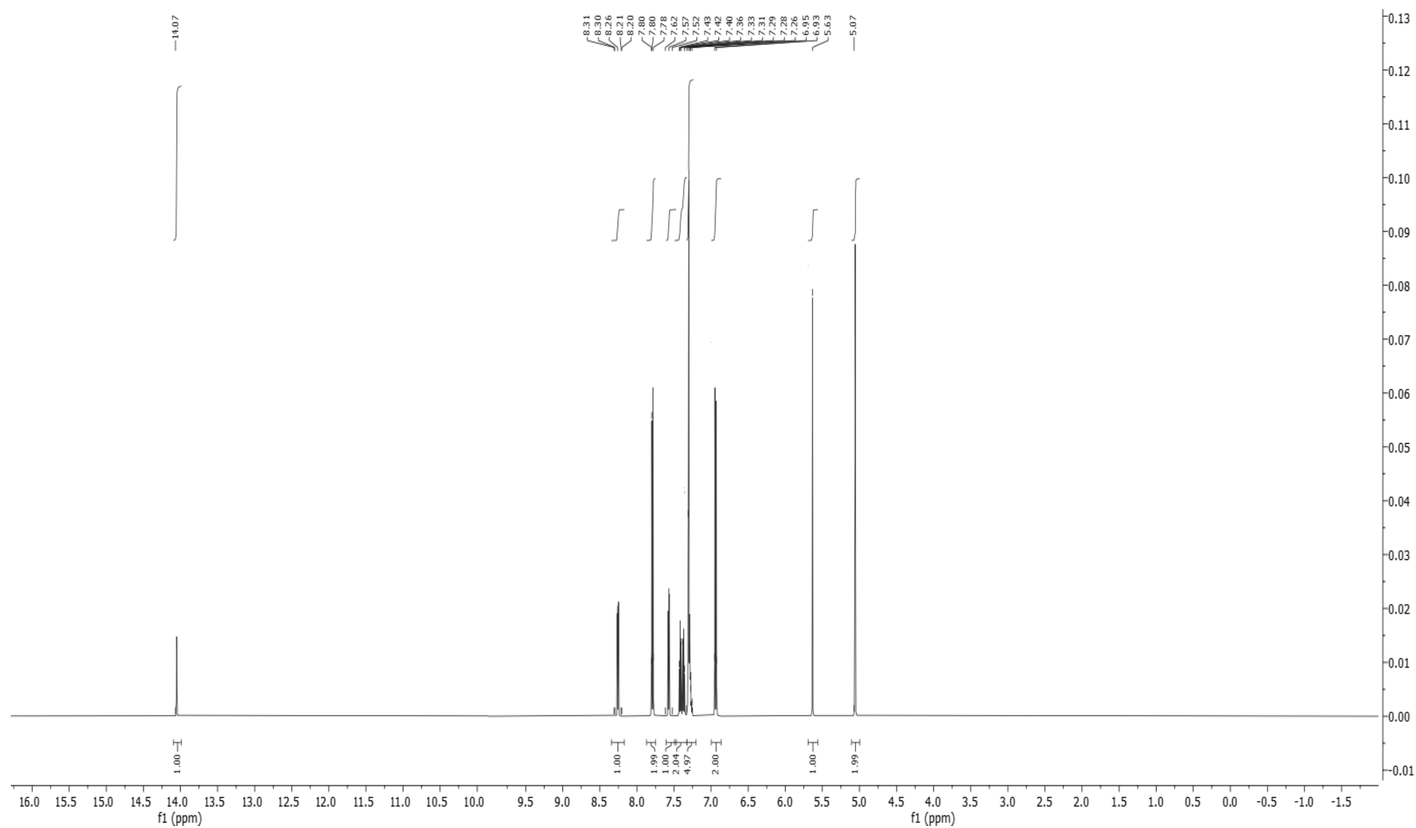
Figure S8: ^1\text{H} NMR spectrum of N'-(1-benzyl-2-oxo-1,2-dihydro-3H-indol-3-ylidene)-2-hydroxybenzohydrazide (5d)
