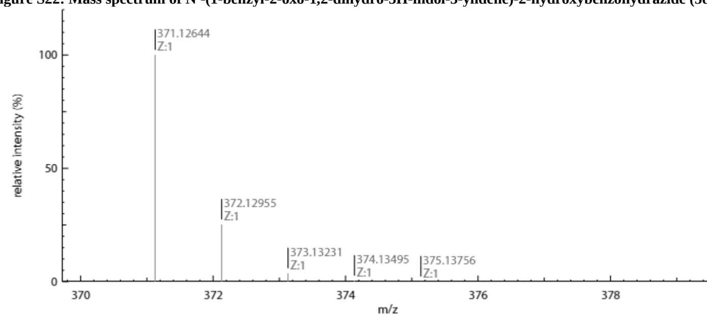
Figure S22: Mass spectrum of N'-(1-benzyl-2-oxo-1,2-dihydro-3H-indol-3-ylidene)-2-hydroxybenzohydrazide (5d)
