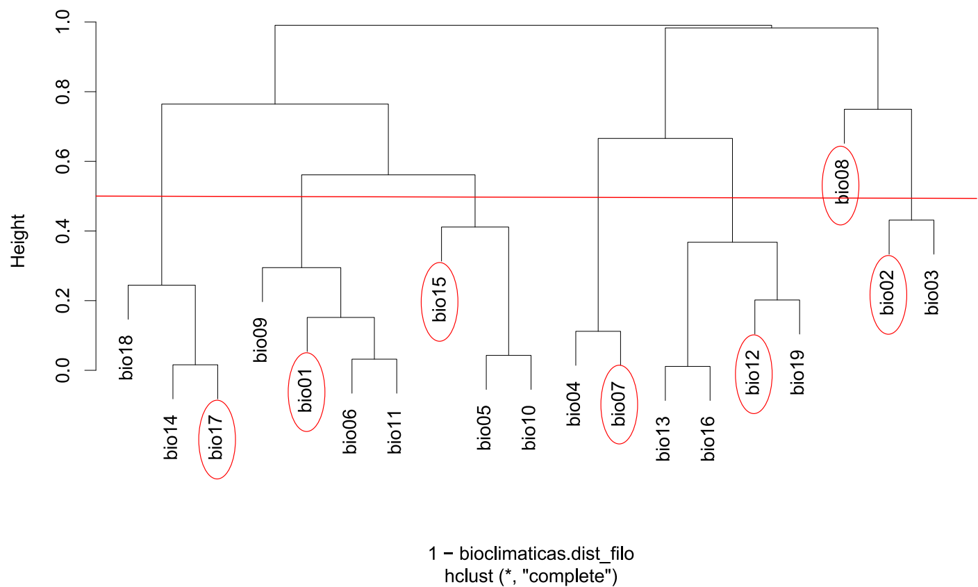
Cluster Dendrogram
