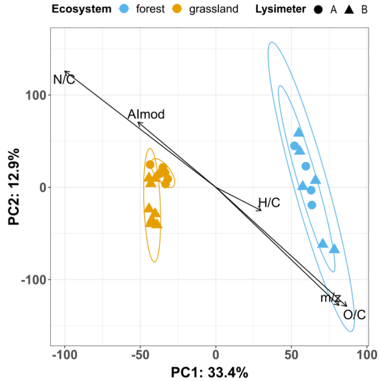
Figure 1. Principal component analysis (PCA) graph based on the molecular composition of DOM samples
