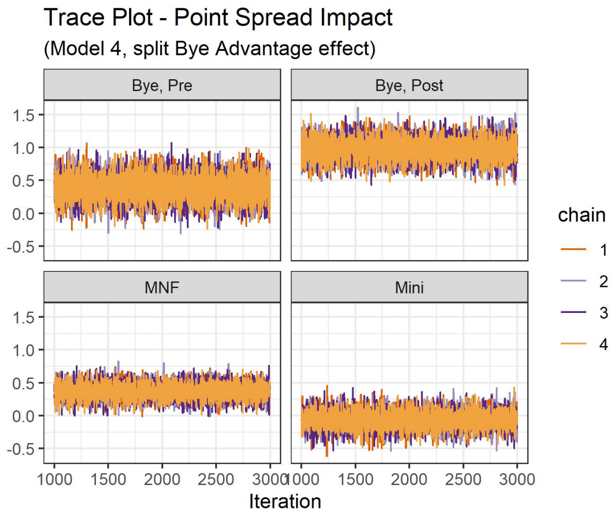
Figure 4. Trace plot for each rest parameter of interest for Model ???. There is no evidence of a lack of convergence.
