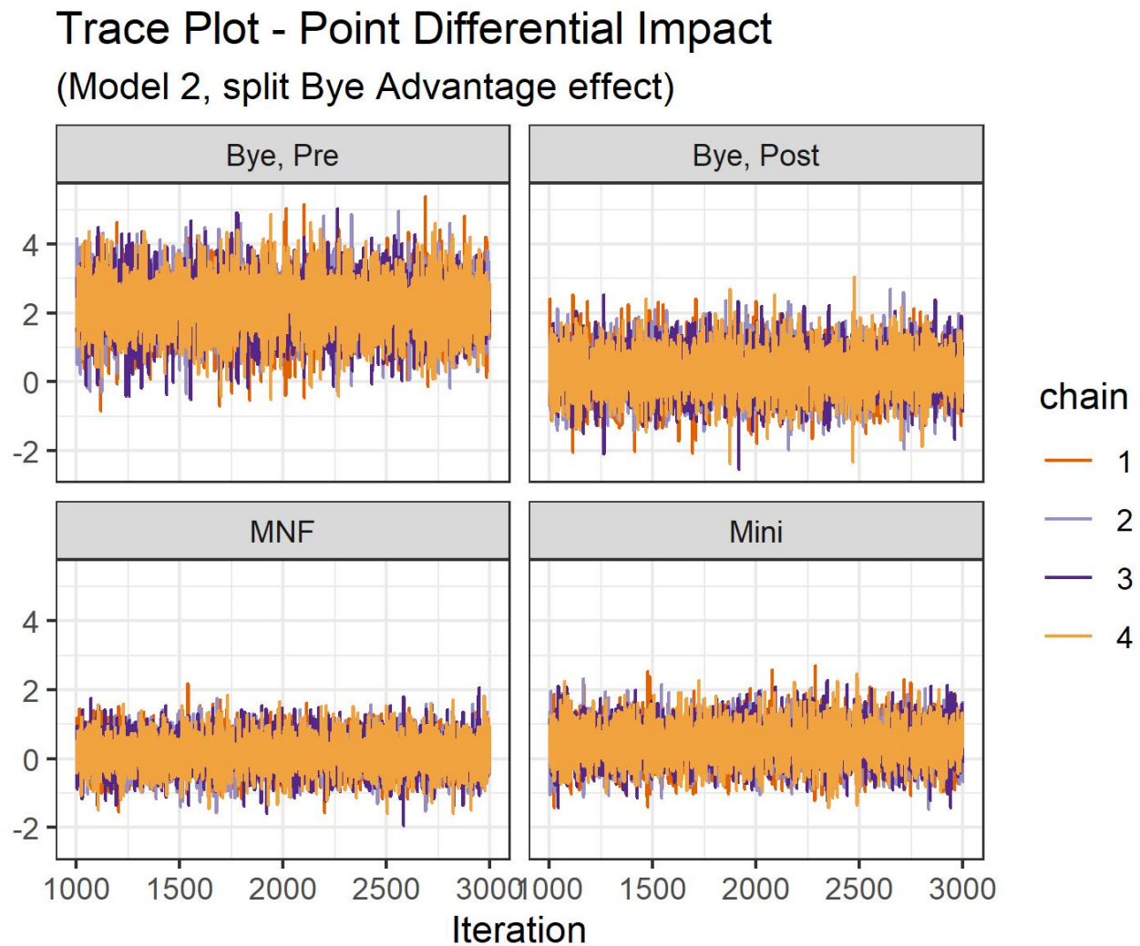
Figure 2. Trace plot for each rest parameter of interest for Model ???. There is no evidence of a lack of convergence.
