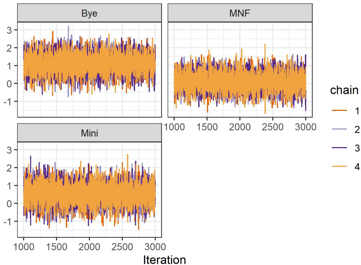
Figure 1. Trace plot for each rest parameter of interest for Model ???. There is no evidence of a lack of convergence.
