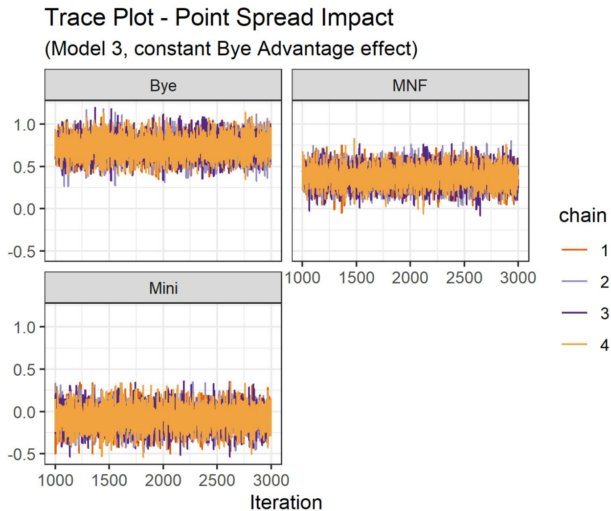
Figure 3. Trace plot for each rest parameter of interest for Model ???. There is no evidence of a lack of convergence.
