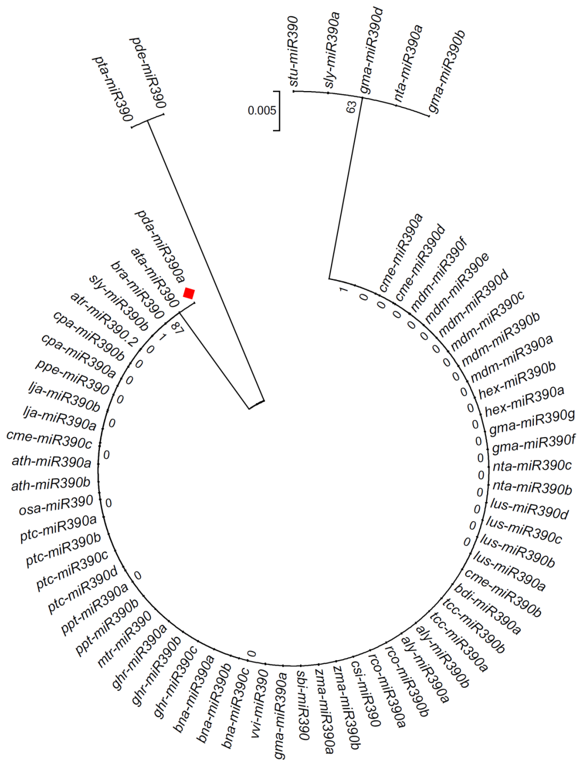
Figure S6. Phylogenetic analysis of the miRNA390 sequences. The phylogenetic tree showed the relationship between the miRNA sequenced from date palm (marked in red colour) and those previously sequenced from other plant species.
