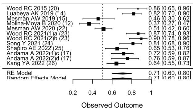
Forest Plot for Sensitivity(metafor) Heterogeneity ( I^2 ): 87.83 %
