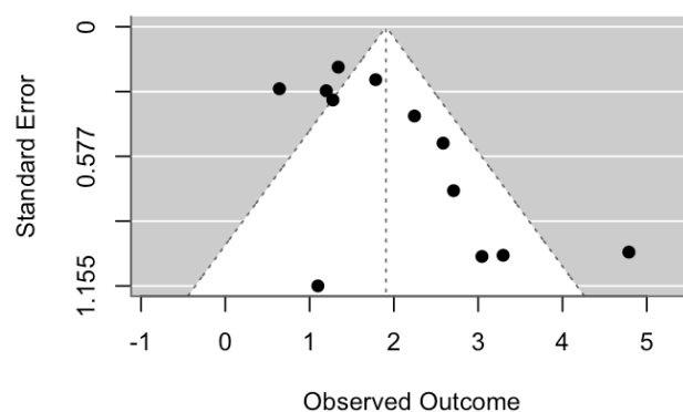
Funnel Plot for Specificity(metafor)
