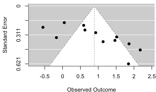
Funnel Plot for Sensitivity(metafor)
