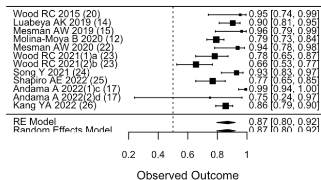
Forest Plot for Specificity(metafor) Heterogeneity ( I^2 ): 82.01 %
