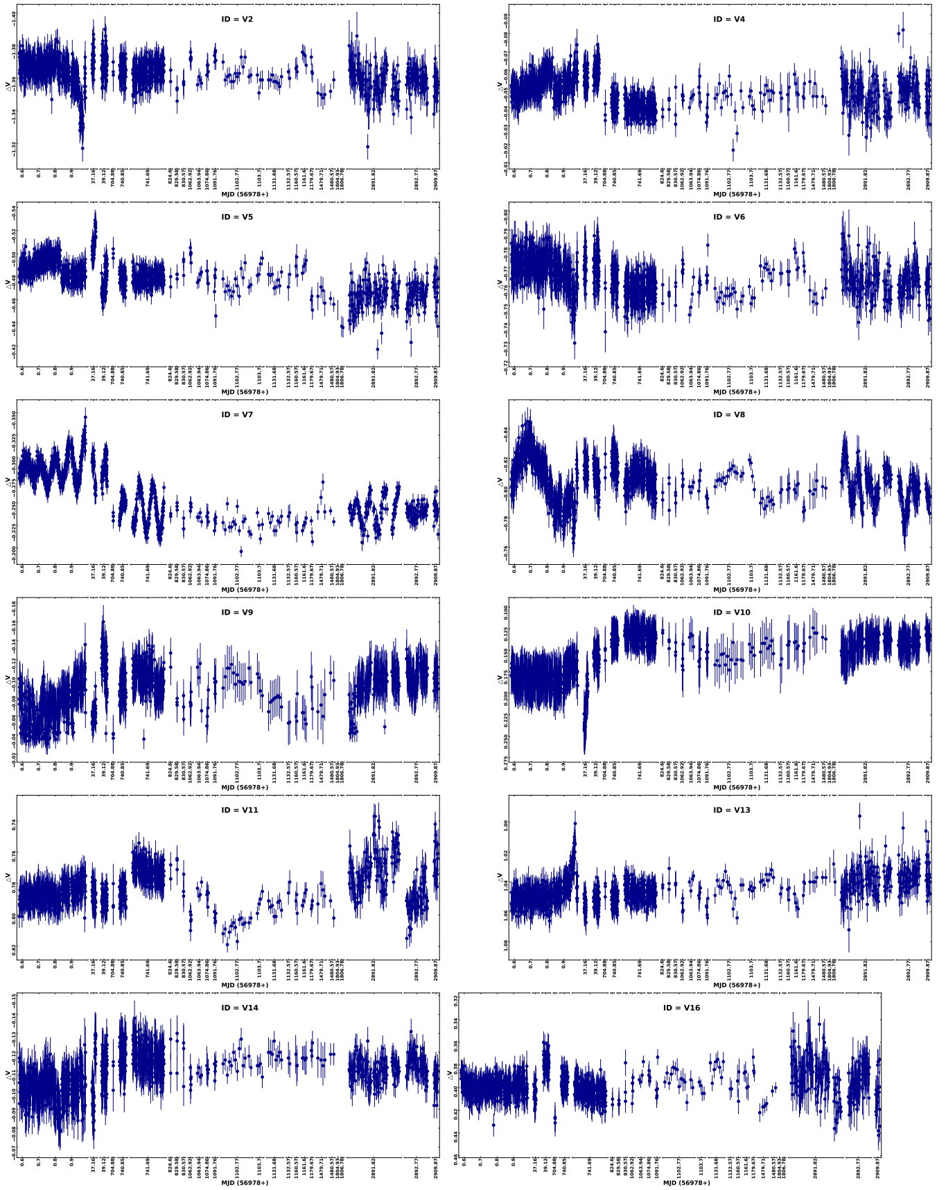
Figure S3. Light curves of periodic variable stars
