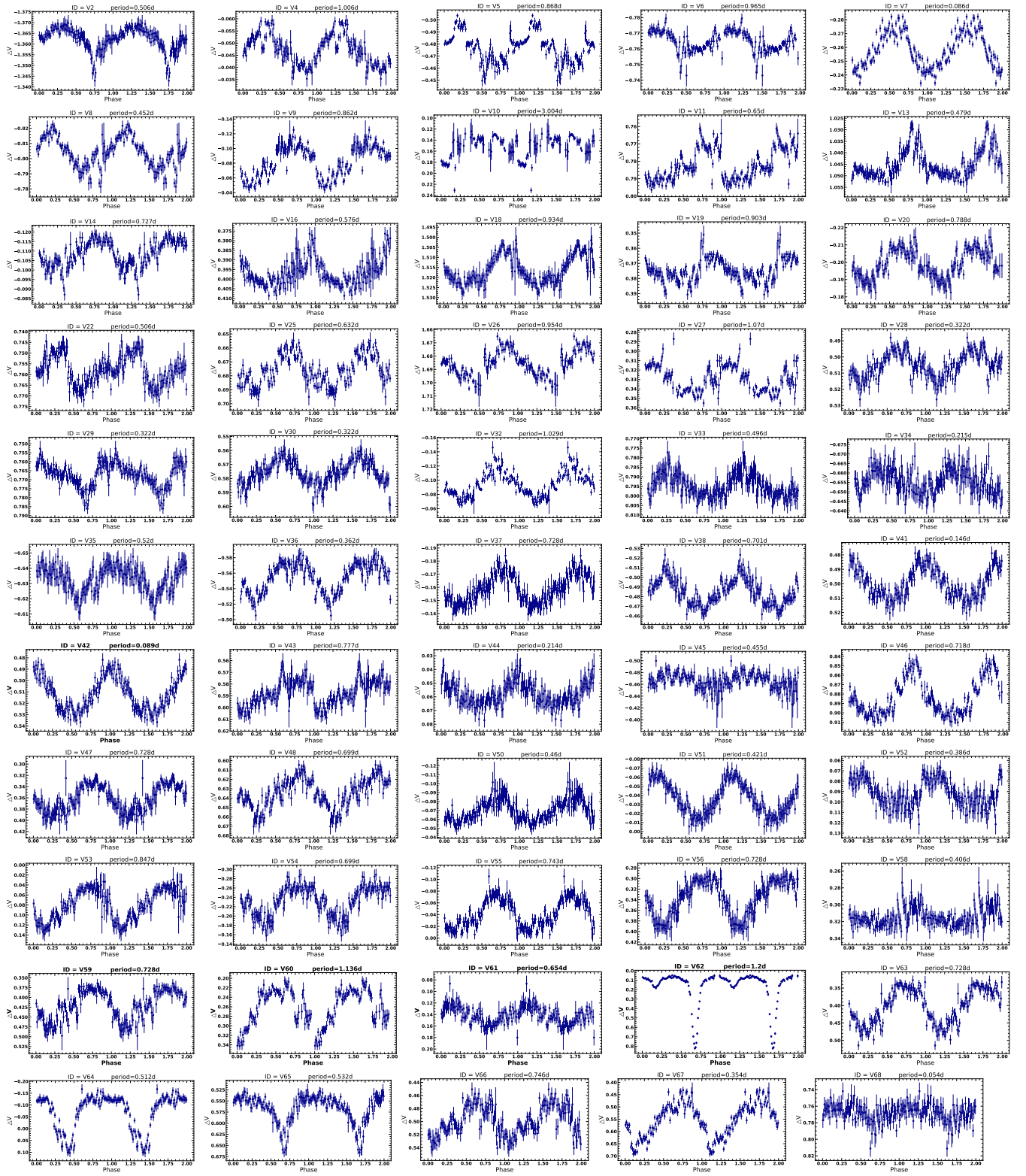
Figure S1. Phase-folded light curves of periodic variable stars
