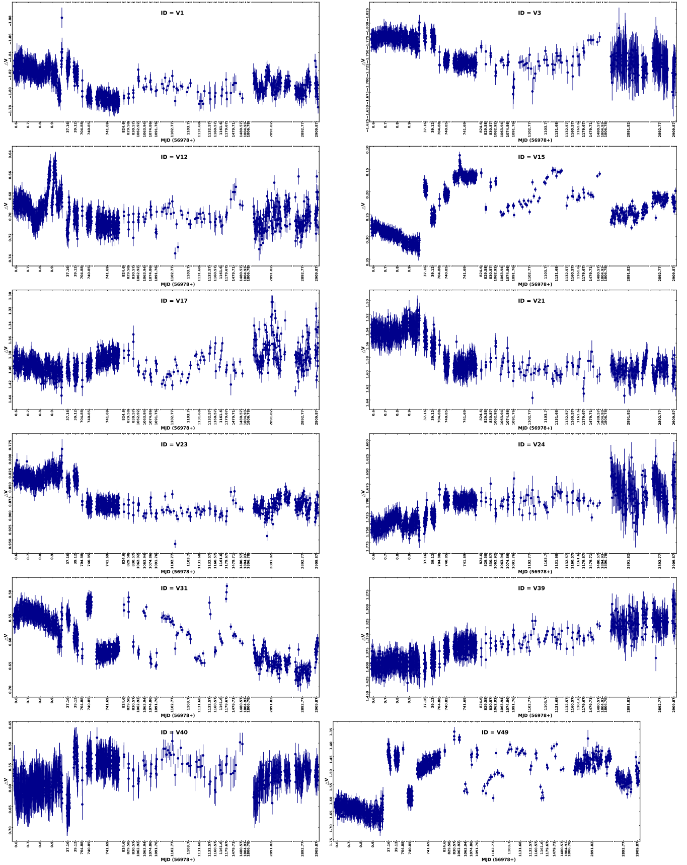
Figure S9. Light curves of non-periodic variables
