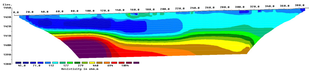
Supplementary Figure 2. ERT profile 4 (autumn 2023)
