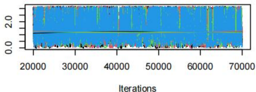
Trace of sd.d
