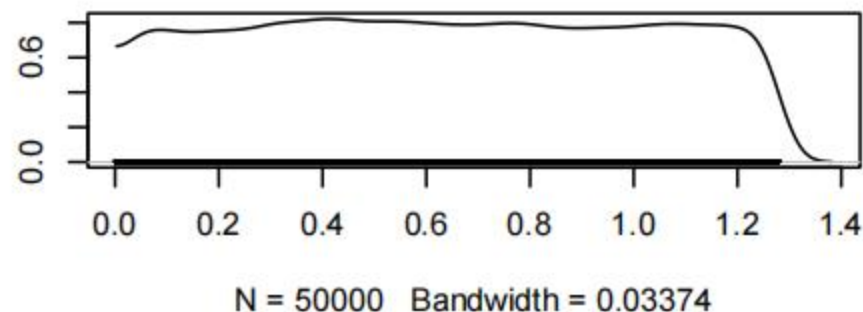
Density of sd.d
