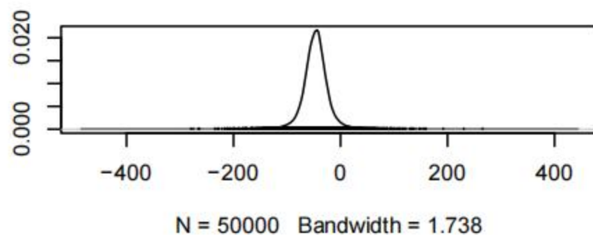
Density of d.1.5
