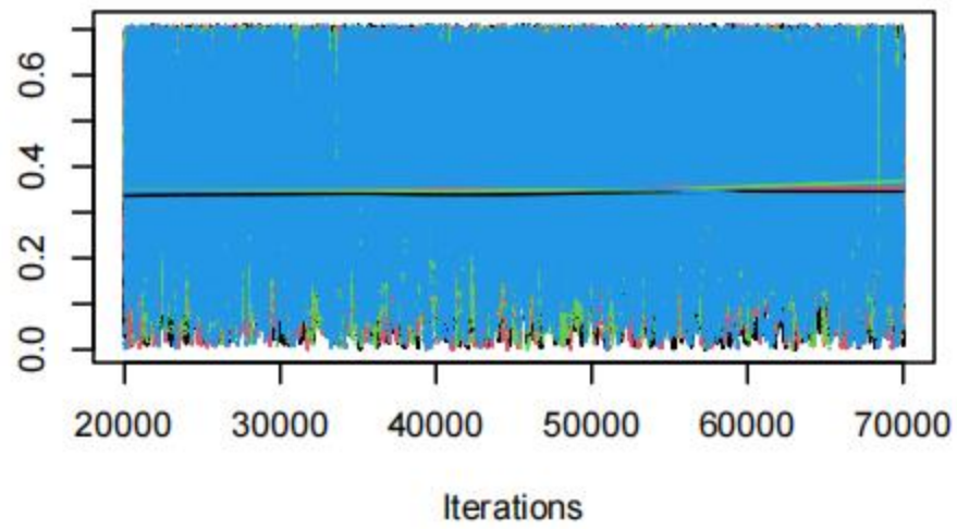
Trace of sd.d
