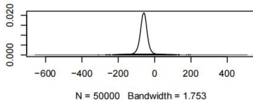
Density of d.1.3
