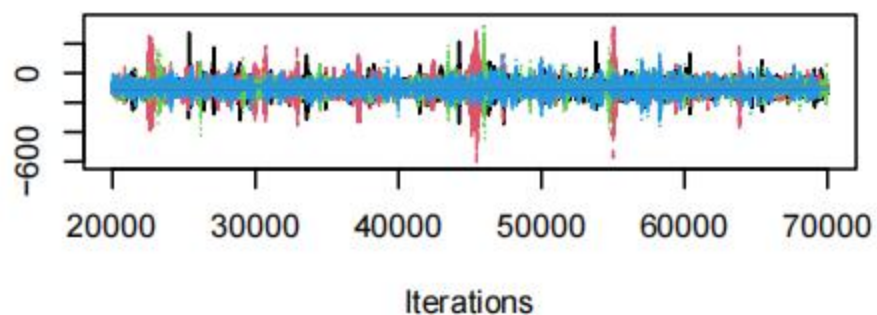
Trace of d.1.8
