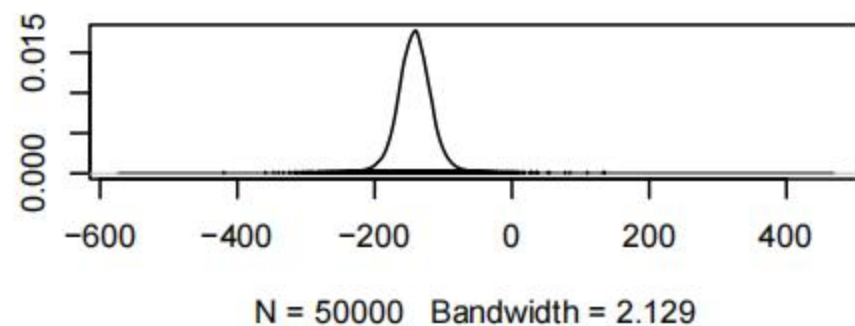
Density of d.1.23
