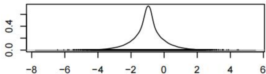
Density of d.1.9
