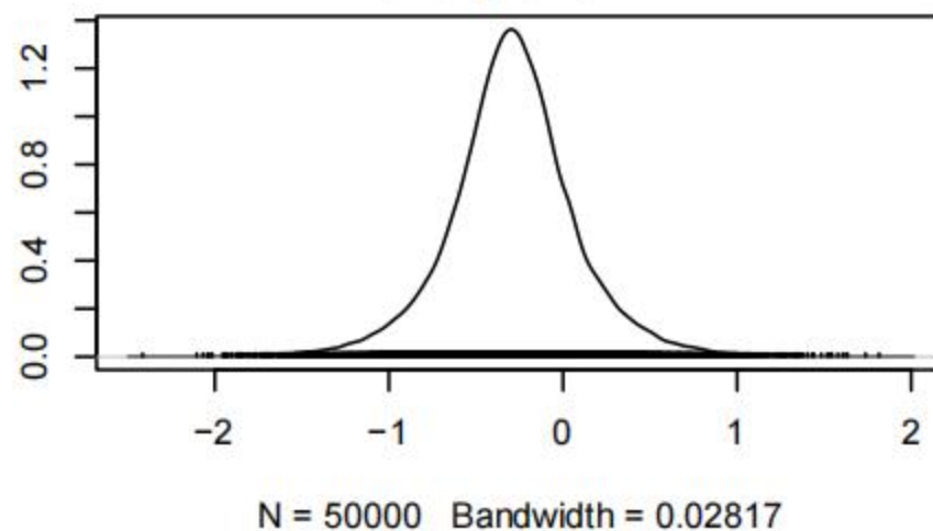
Density of d.1.14
