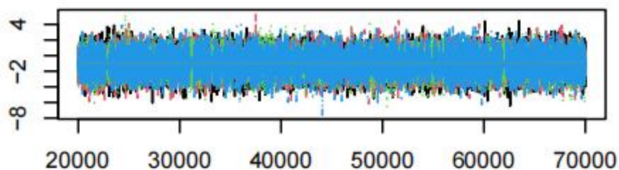
Trace of d.1.9
