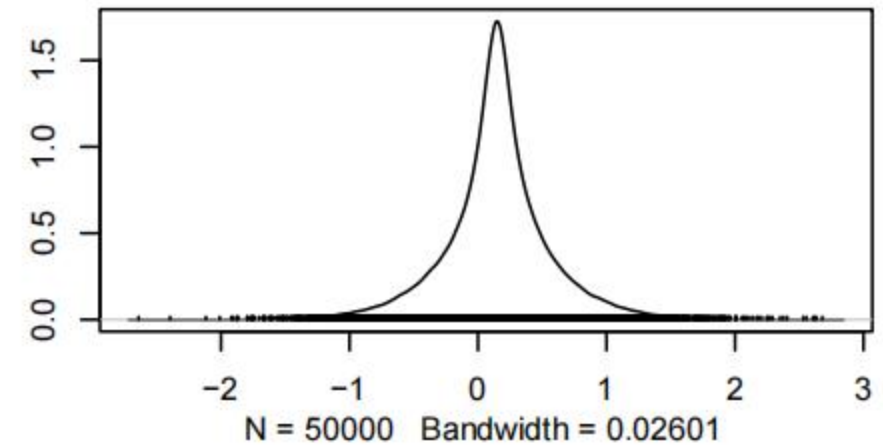
Density of d.1.15
