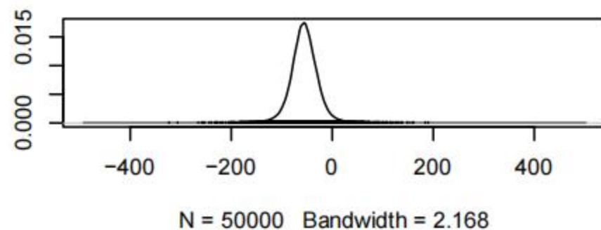
Density of d.1.24
