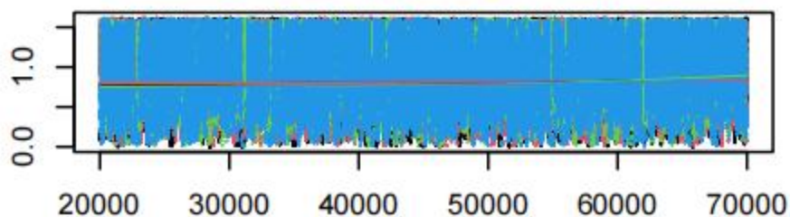
Trace of sd.d
