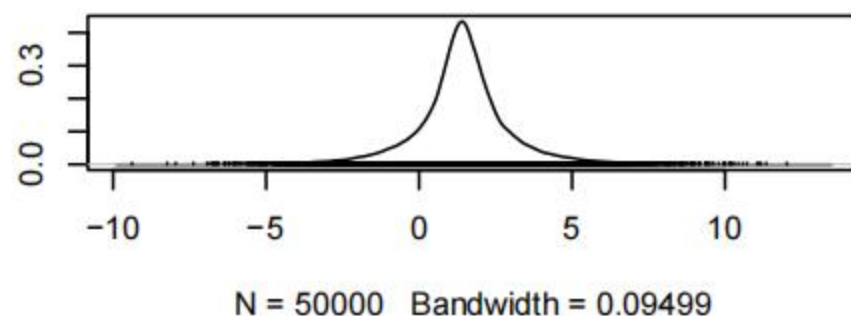
Density of d.1.9
