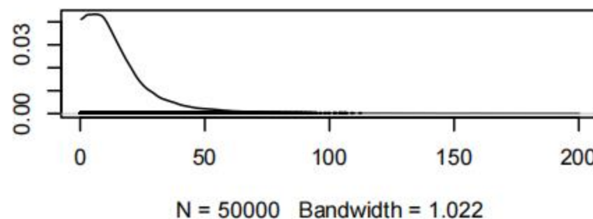
Density of sd.d
