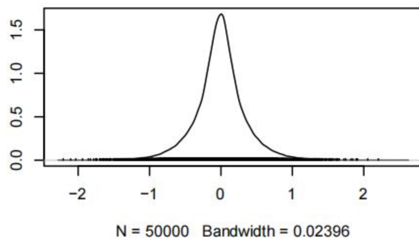
Density of d.1.27
