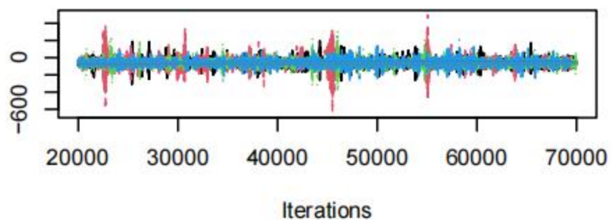
Trace of d.1.3
