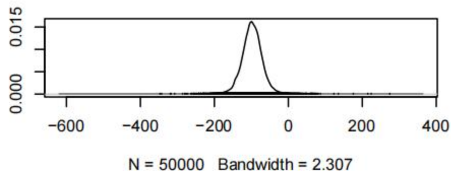
Density of d.1.8
