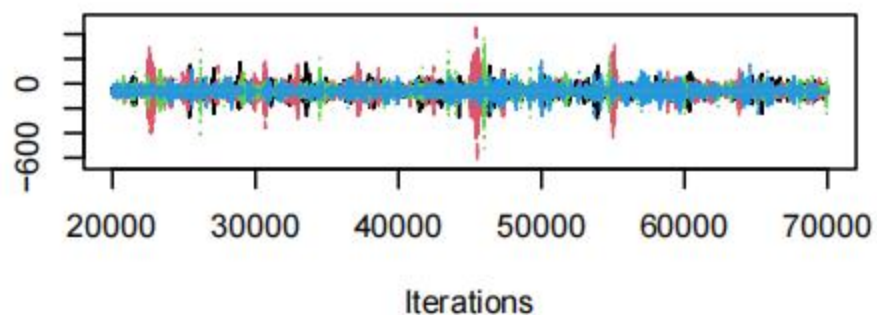
Trace of d.1.9
