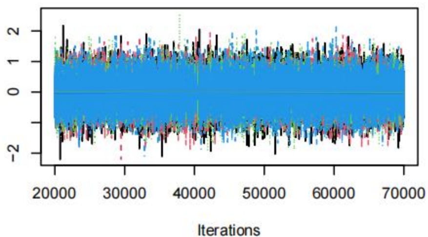
Trace of d.1.27
