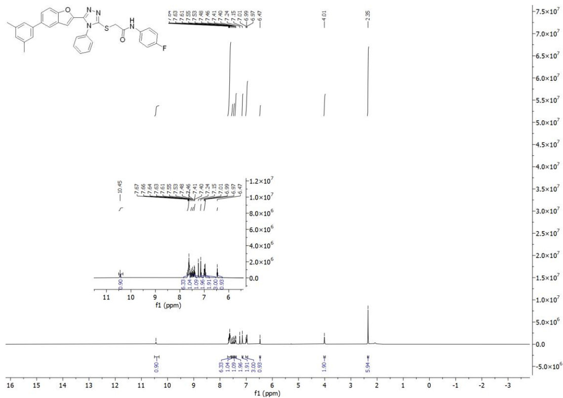
Figure S 1.17: ^1\text{H} -NMR Spectra of compound 13i .
