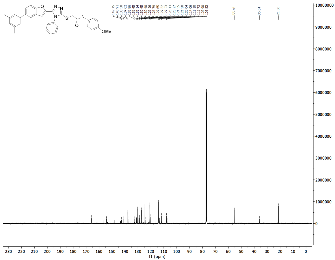
Figure S 1.10: ^{13}\text{C} -NMR Spectra of compound 13e .
