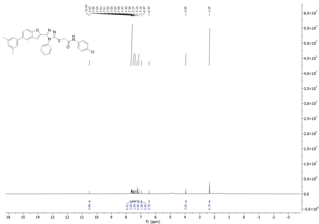
Figure S 1.15: 1 H-NMR Spectra of compound 13h .
