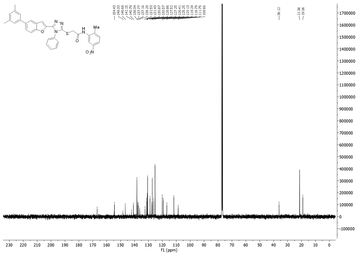
Figure S 1.8: 13 C-NMR Spectra of compound 13d .
