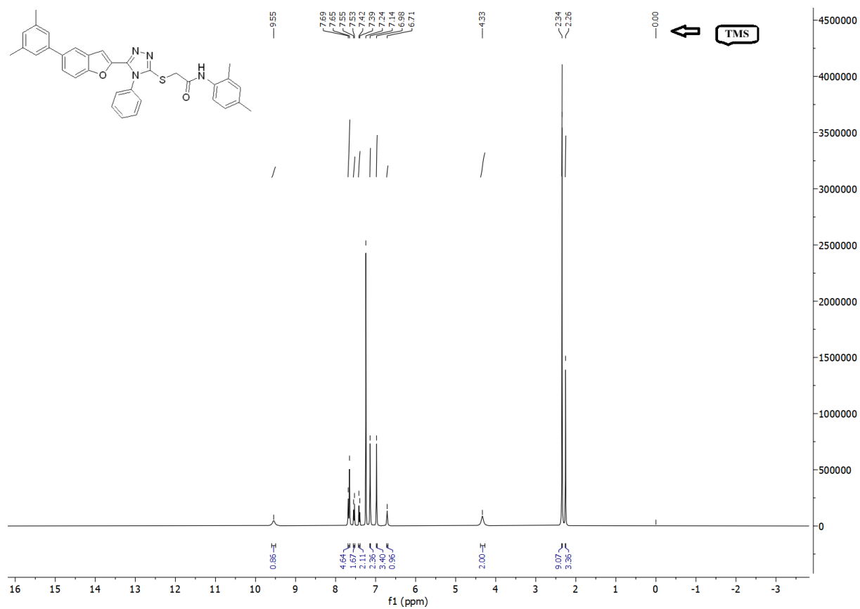
Figure S 1.1: ^1\text{H} -NMR Spectra of compound 13a .
