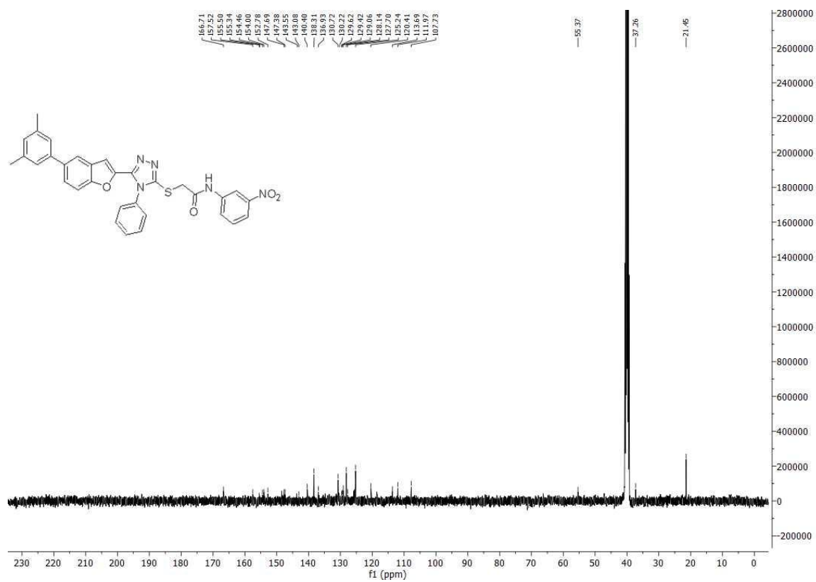
Figure S 1.6: 13 C-NMR Spectra of compound 13c.
