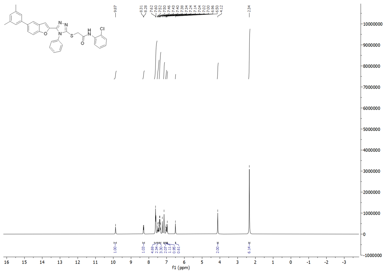
Figure S 1.13: 1 H-NMR Spectra of compound 13g .
