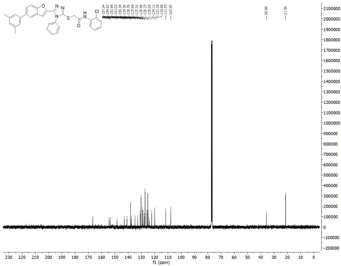
Figure S 1.14: ^{13}\text{C} -NMR Spectra of compound 13g .
