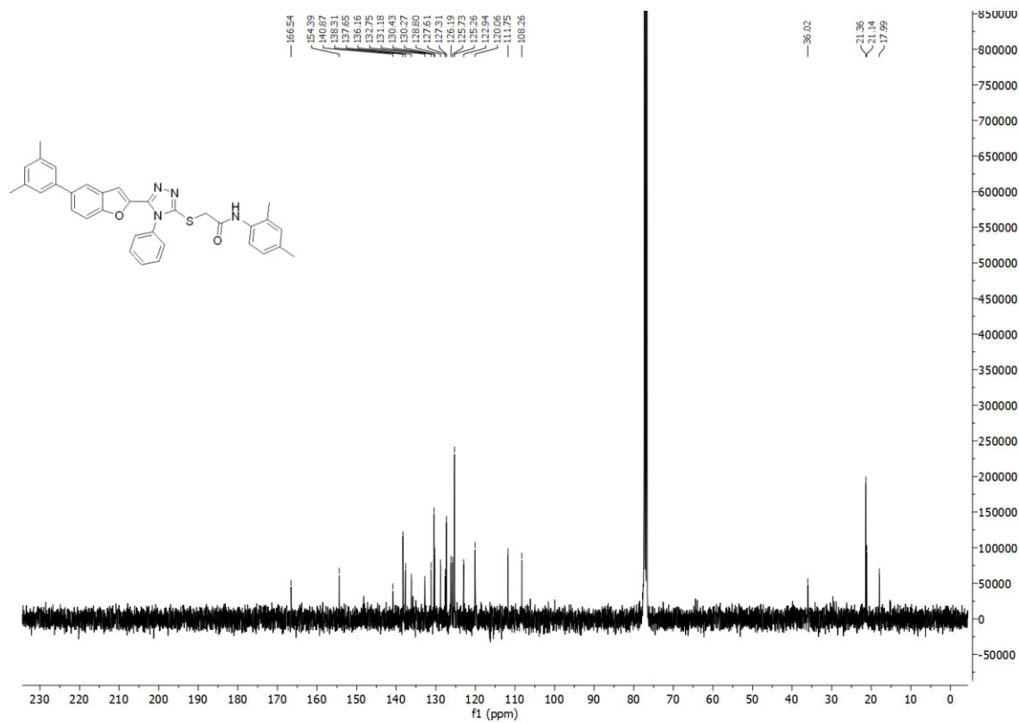
Figure S 1.2: ^{13}\text{C} -NMR Spectra of compound 13a .
