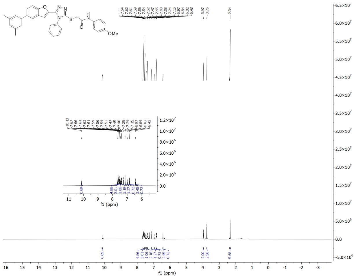
Figure S 1.9: 1 H-NMR Spectra of compound 13e .
