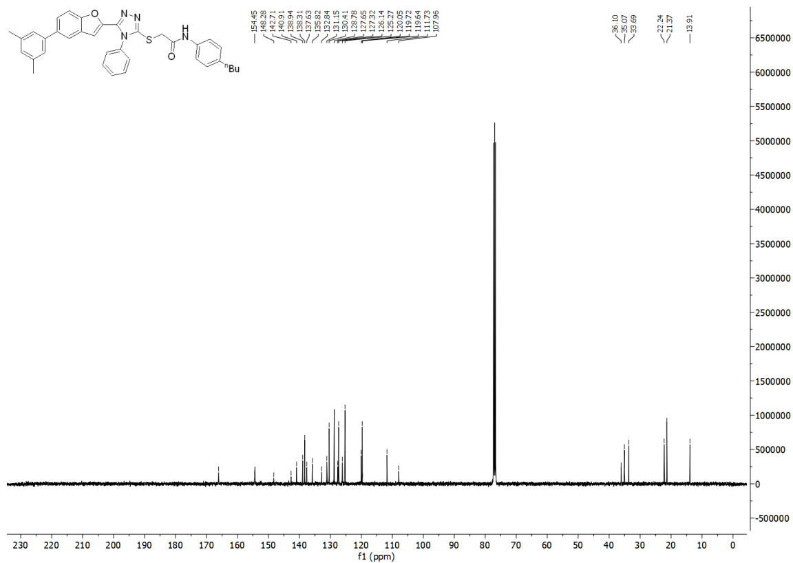
Figure S 1.12: ^{13}\text{C} -NMR Spectra of compound 13f .
