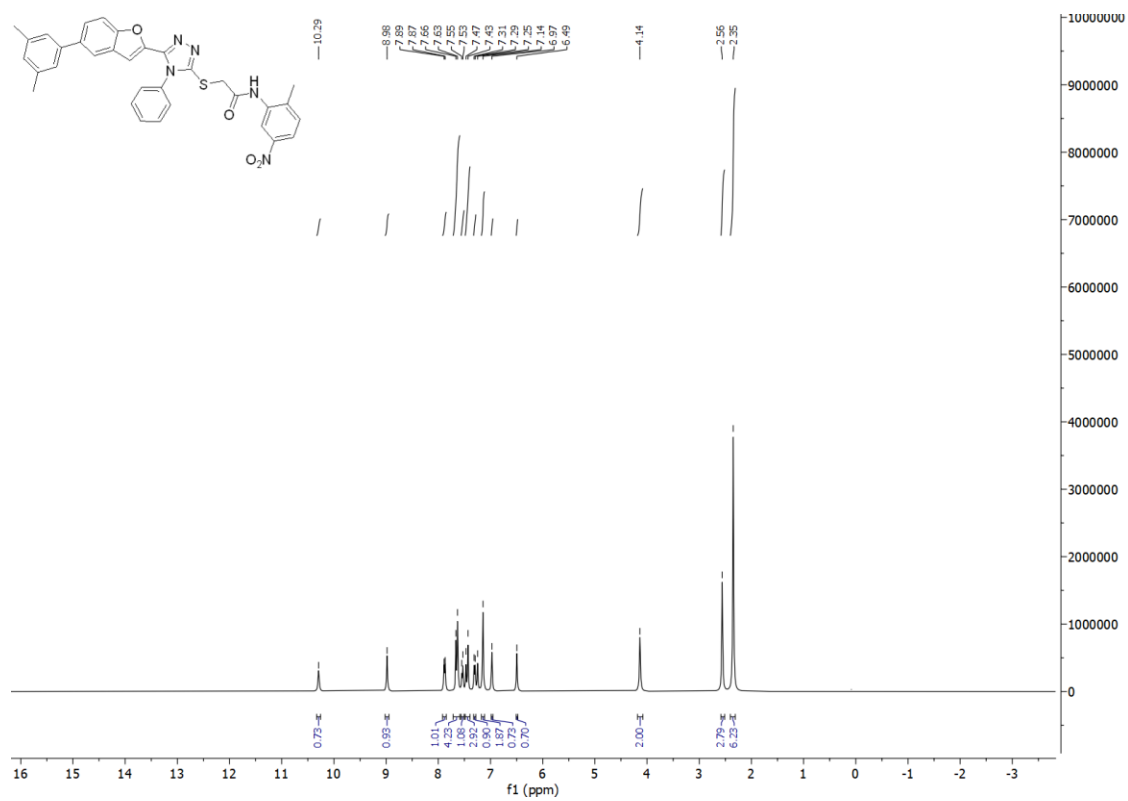
Figure S 1.7: ^1\text{H} -NMR Spectra of compound 13d .
