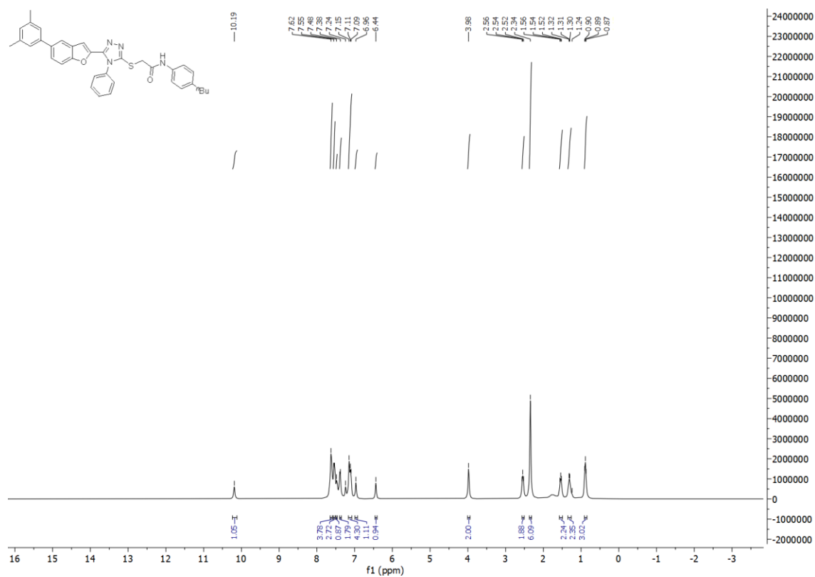
Figure S 1.11: ^1\text{H} -NMR Spectra of compound 13f .
