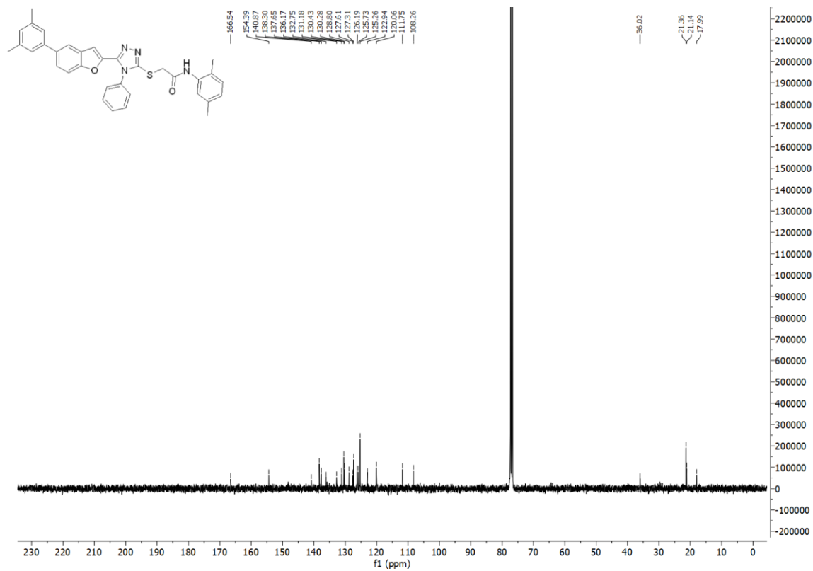
Figure S 1.4: ^{13}\text{C} -NMR Spectra of compound 13b .
