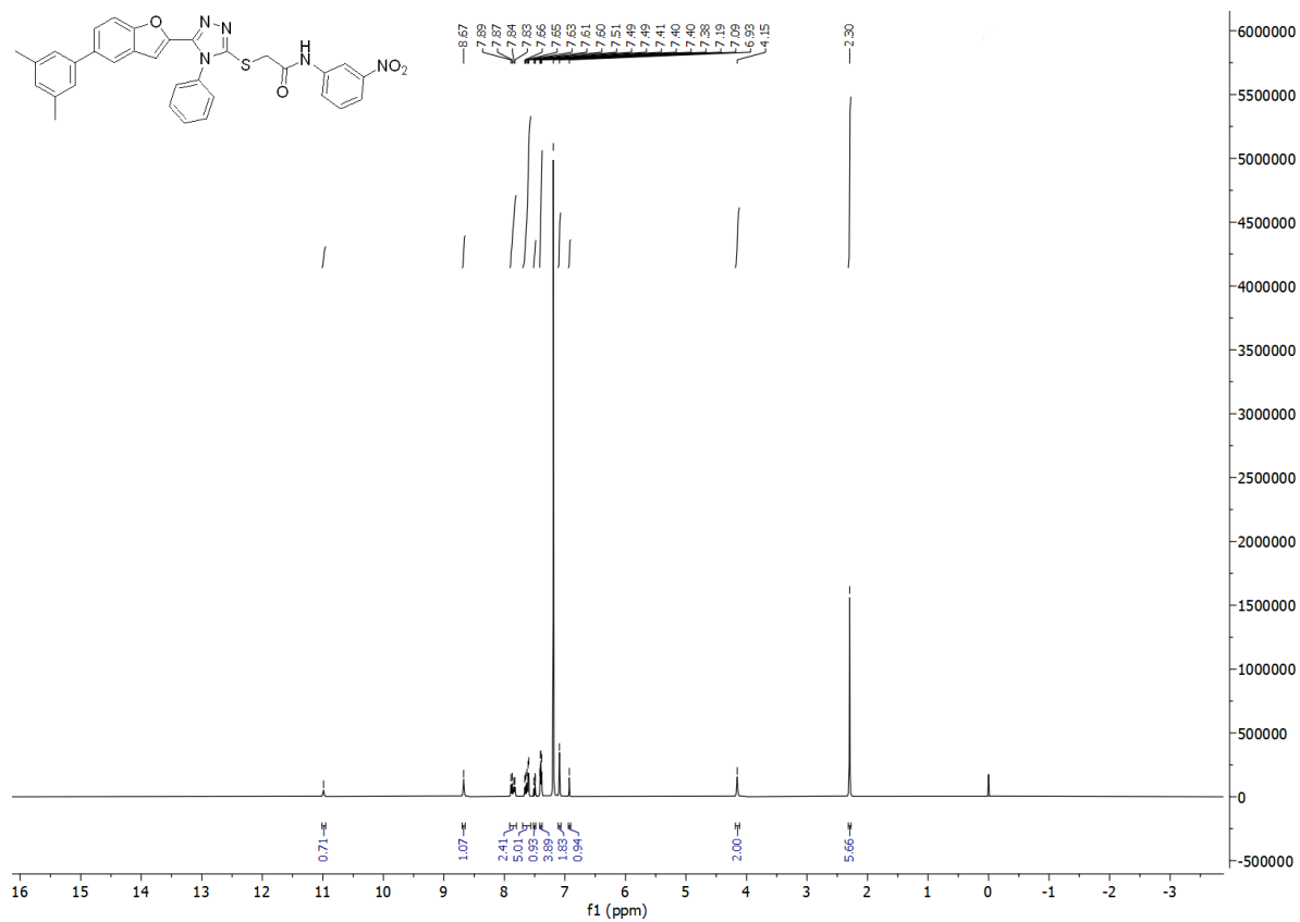
Figure S 1.5: 1 H-NMR Spectra of compound 13c .
