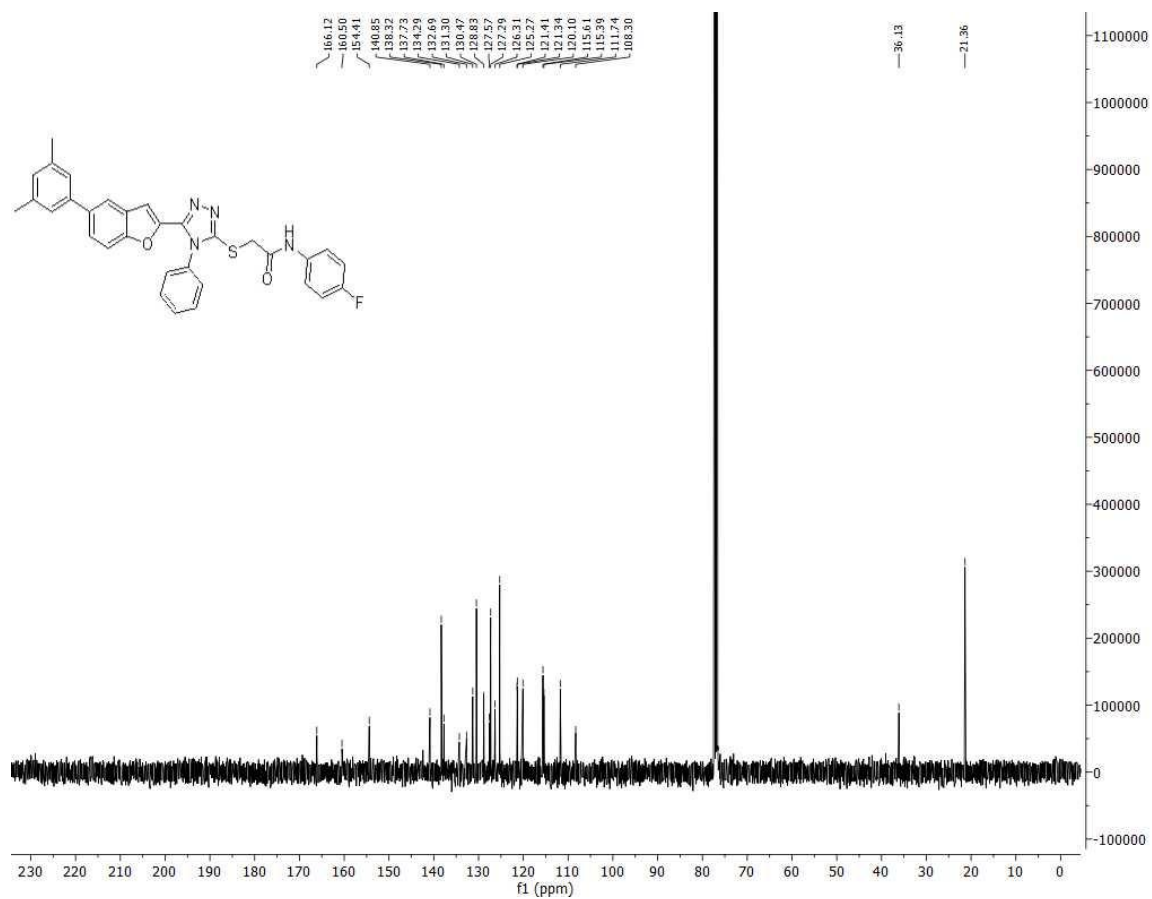
Figure S 1.18: 13 C-NMR Spectra of compound 13i .
