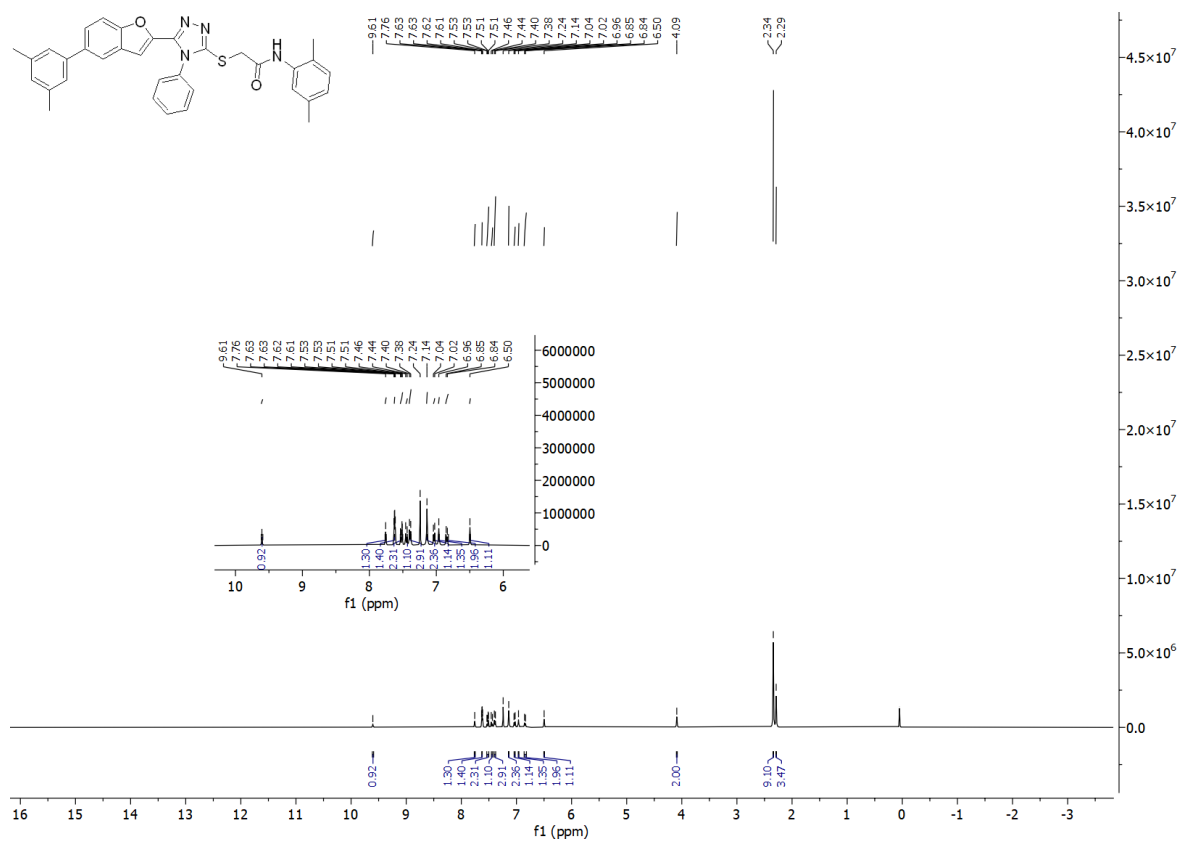
Figure S 1.3: ^1\text{H} -NMR Spectra of compound 13b .
